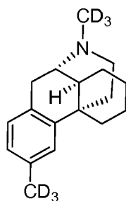
Compound 110.
