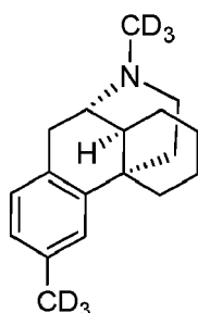
Compound 110.
