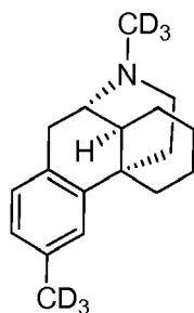
Compound 110,
