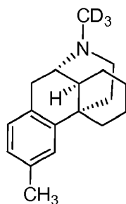
Compound 109,
