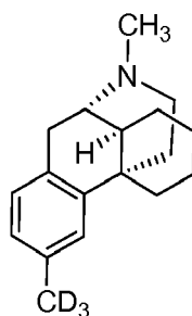
Compound 108,
