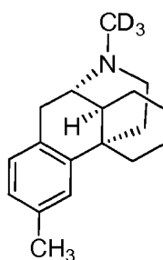
Compound 109, and
