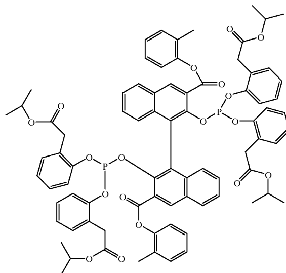
Ligand 1
