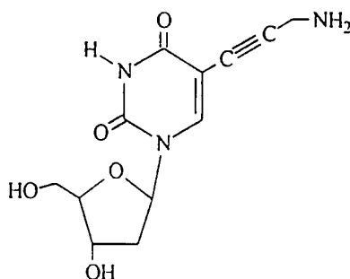
5-(3-aminoprop-1-yn-1-yl)-2'-deoxyuridine
