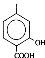
Chelating group
