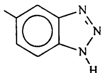
Bridging ligand
