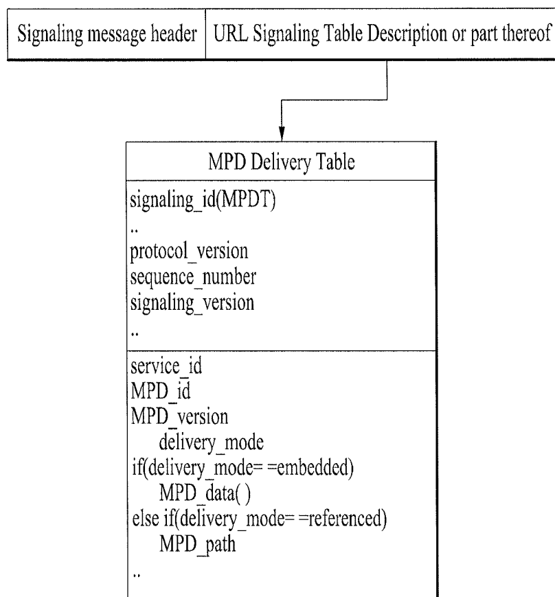
MDP Delivery Table Description Semantics
