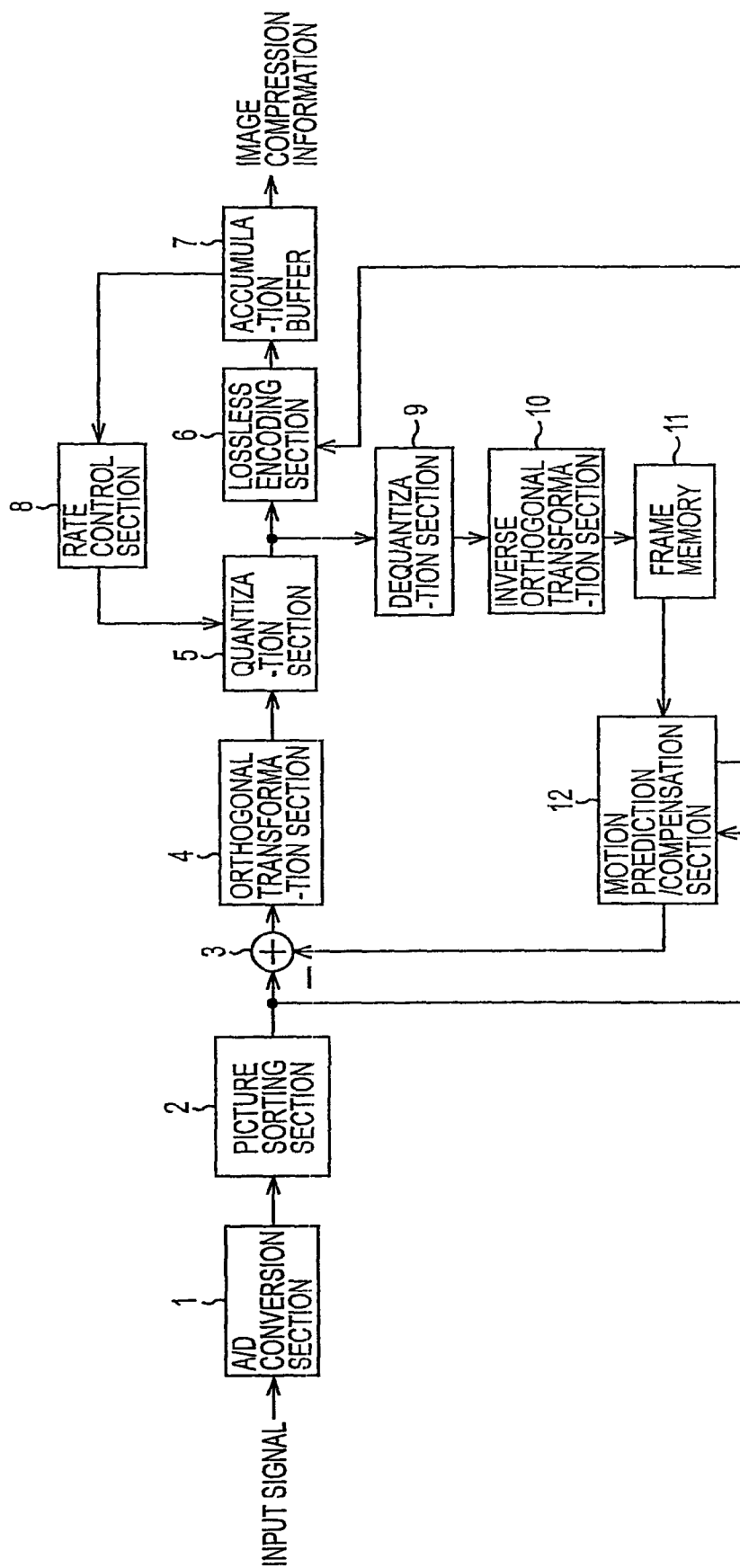
FIG. 1 BACKGROUND ART
