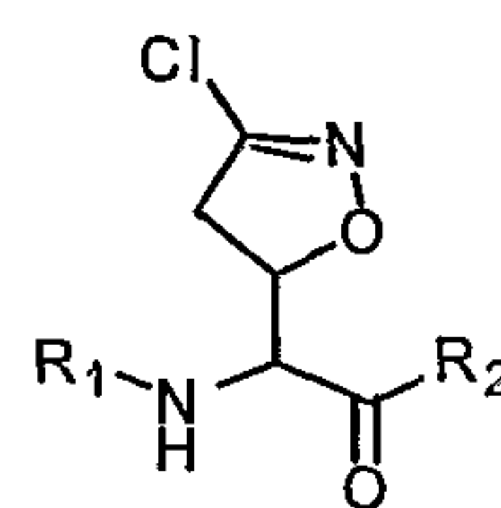
3-halo-4,5-dihydroisoxazoles
