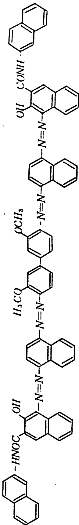
Structural Formula
