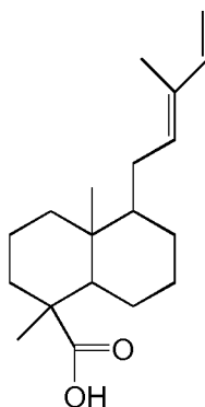
Labane acid
