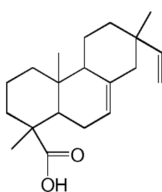
Isopimaric acid
