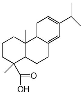
Levopimaric acid
