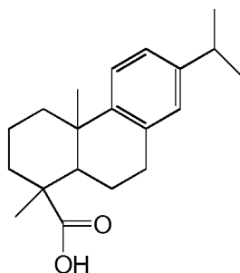
Dehydroabietic acid
