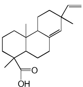
Pimaric acid
