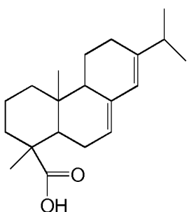
10 Abietic acid
