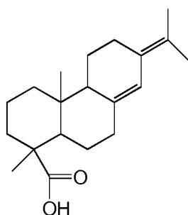
Neoabietic acid
