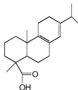
Palustric acid
