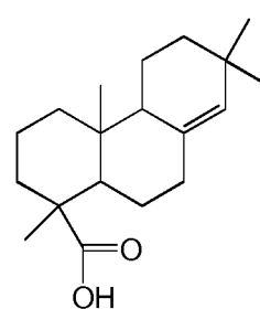
Sandracopimaric acid
