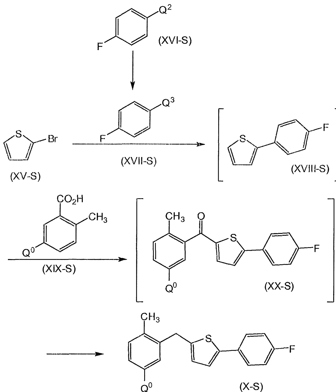
Scheme 4
