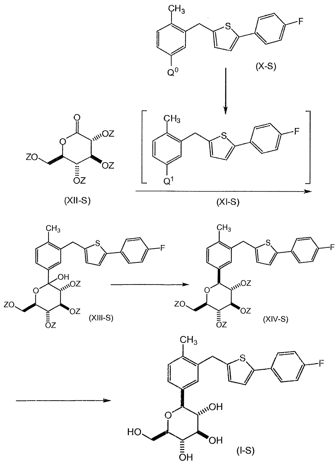
Scheme 2
