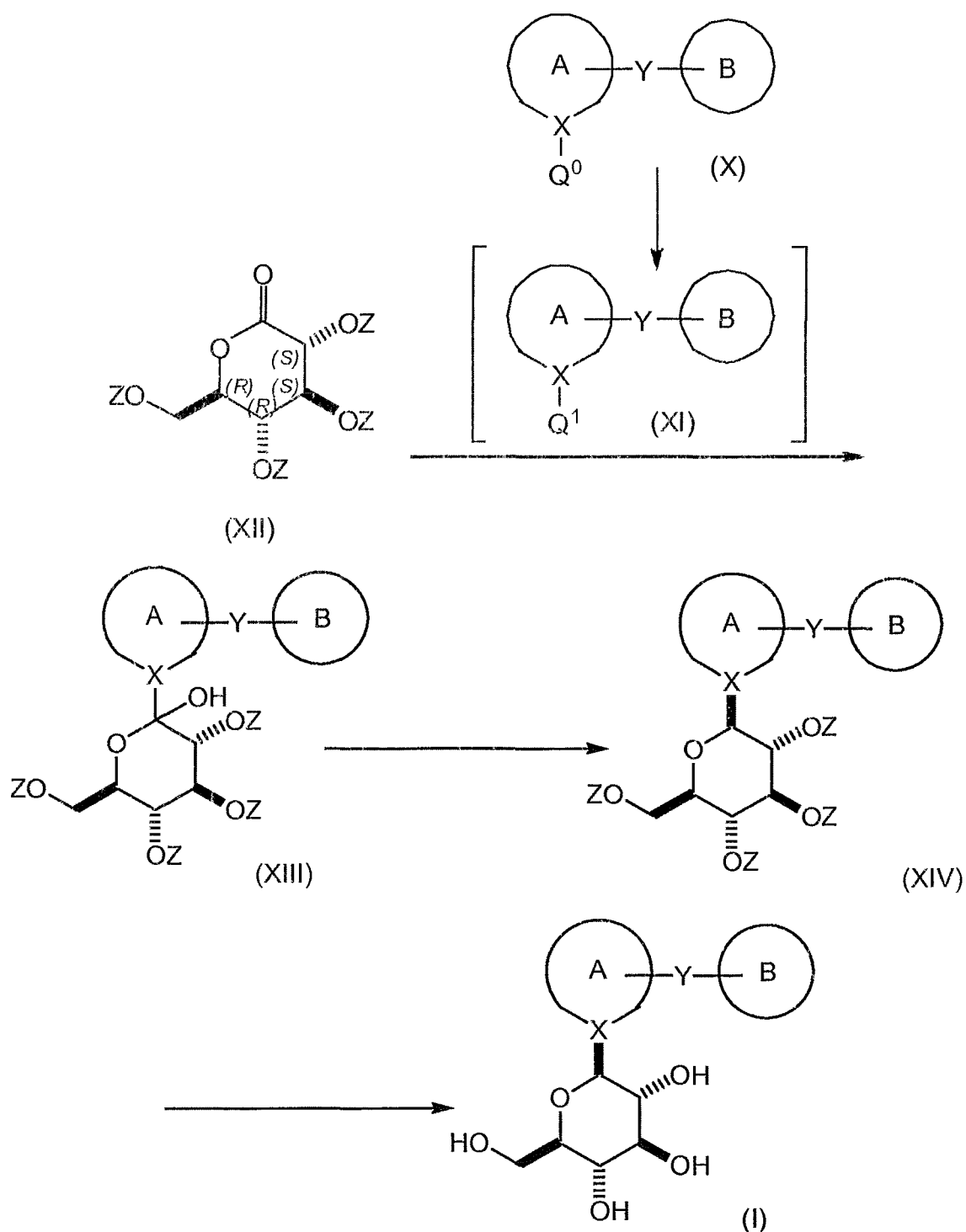
Scheme 1
