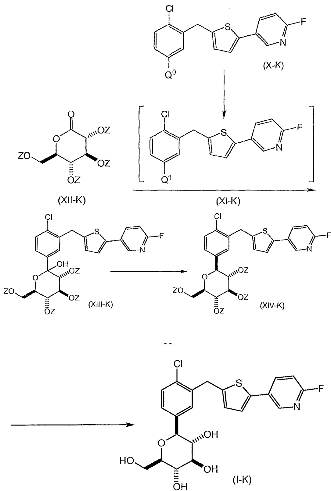
Scheme 3
