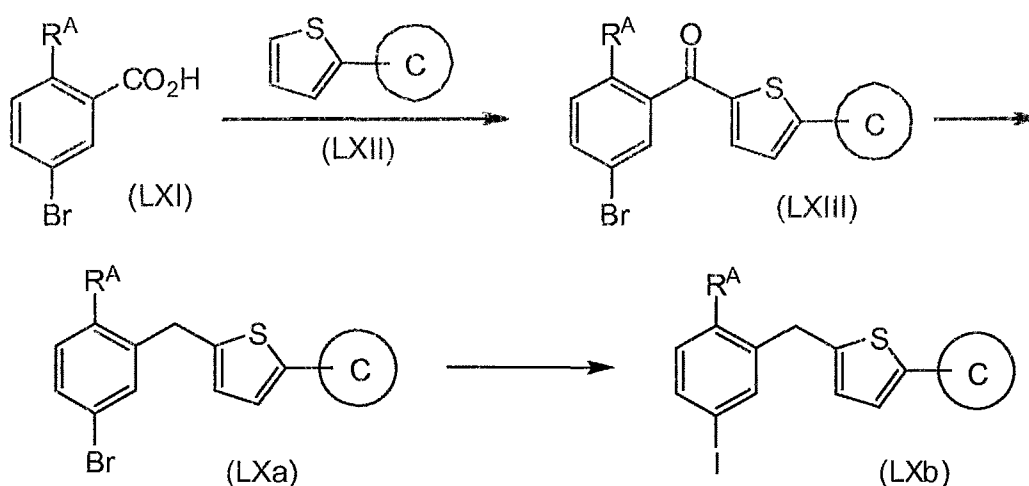
Scheme 9
