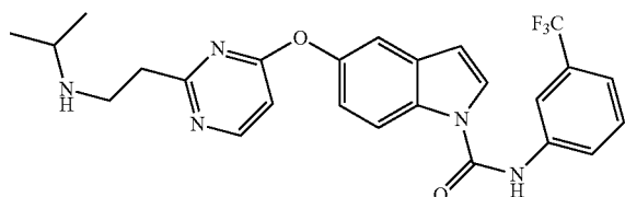
73-K 5-(2-(2-(isopropylamino)ethyl)pyrimidin-4-yloxy)-N-(3-(trifluoromethyl)phenyl)-1H-indole-1-carboxamide
