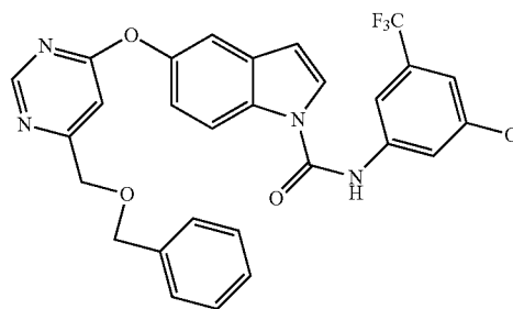
76-A. 5-(6-(benzyloxymethyl)pyrimidin-4-yloxy)-N-(3-methoxy-5-(trifluoromethyl)phenyl)-1H-indole-1-carboxamide
