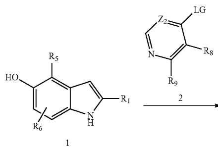
Scheme 1
