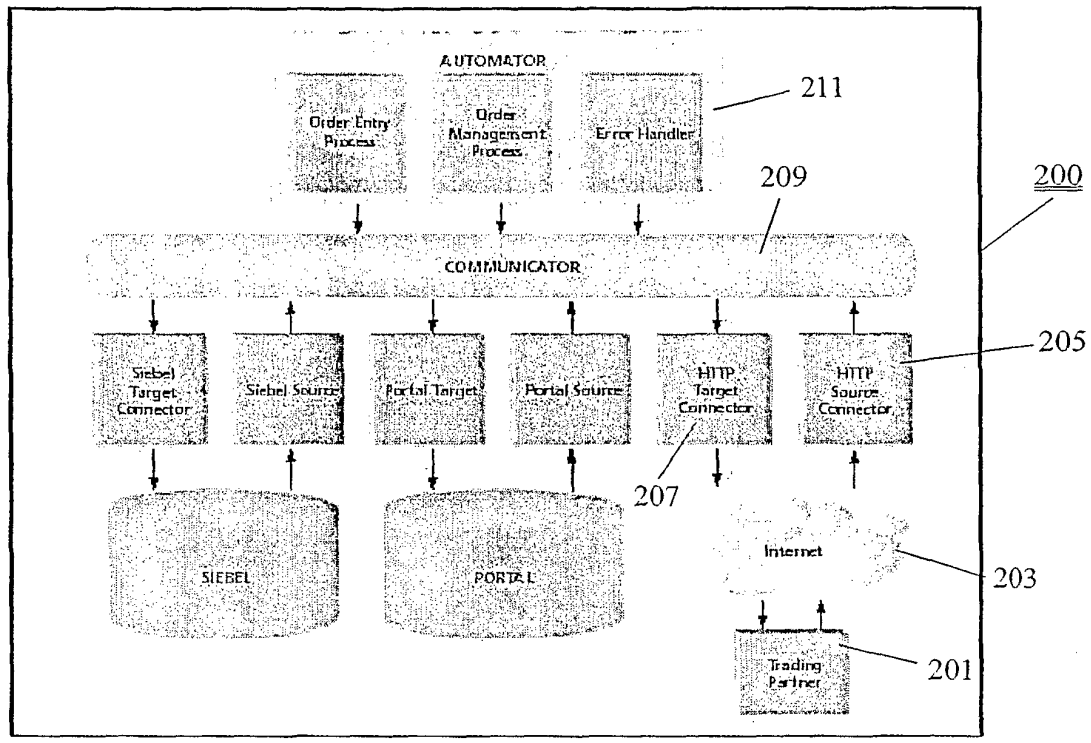
FIGURE 2 SIEBEL-PORTAL TRADING PARTNER INTEGRATION ARCHITECTURE PRIOR ART
