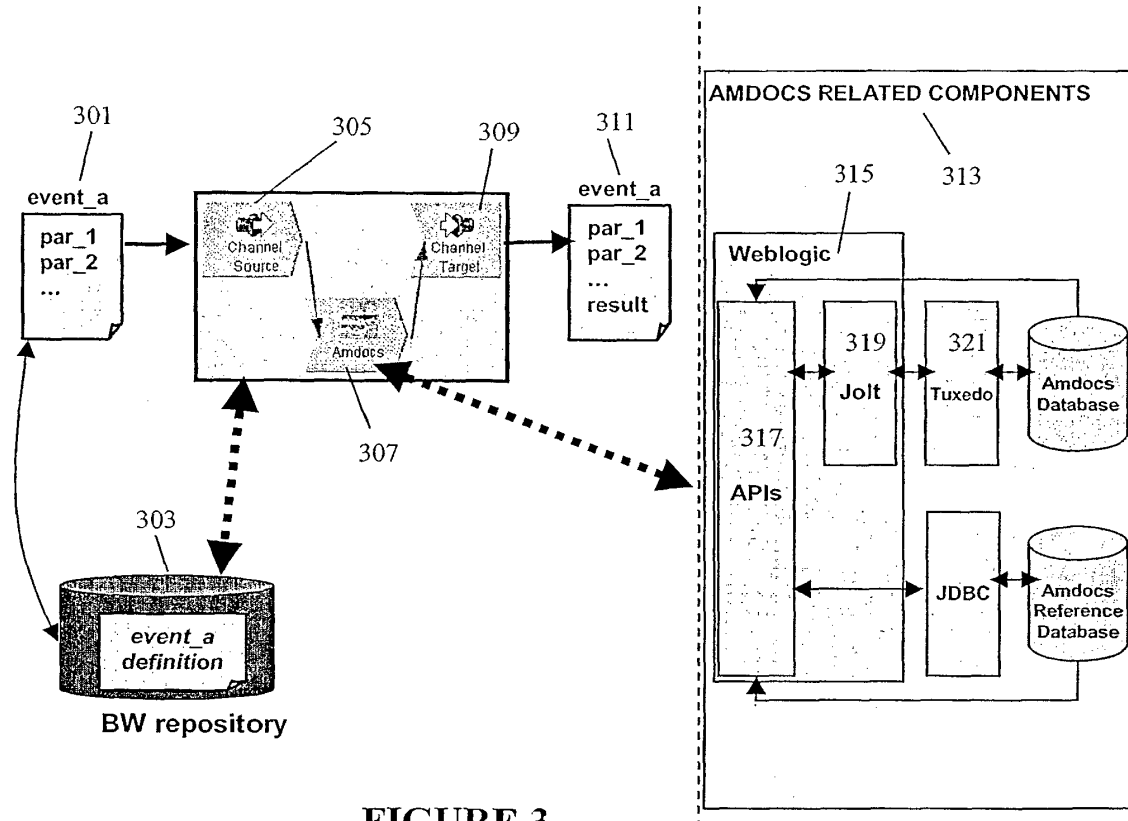
FIGURE 3 Vitria EJB/Amdocs Connector
