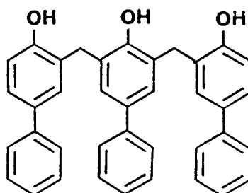
p -phenyl-phenol formaldehyde polymer
