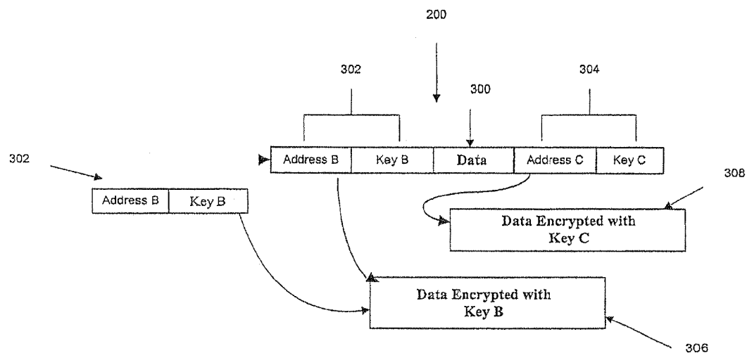
Figure 6. Discarding crypto-pointer A makes Data and the C structure forever inaccessible
