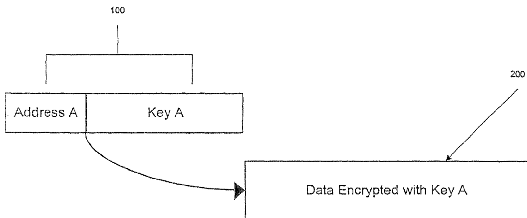
Figure 2. Crypto-pointer always points to cell encrypted with associated key
