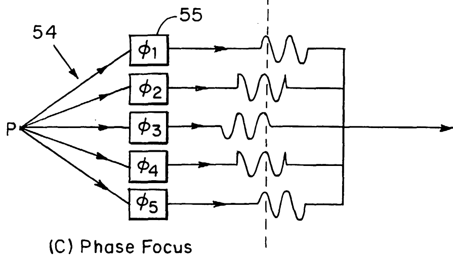
FIG. 2C Prior Art
