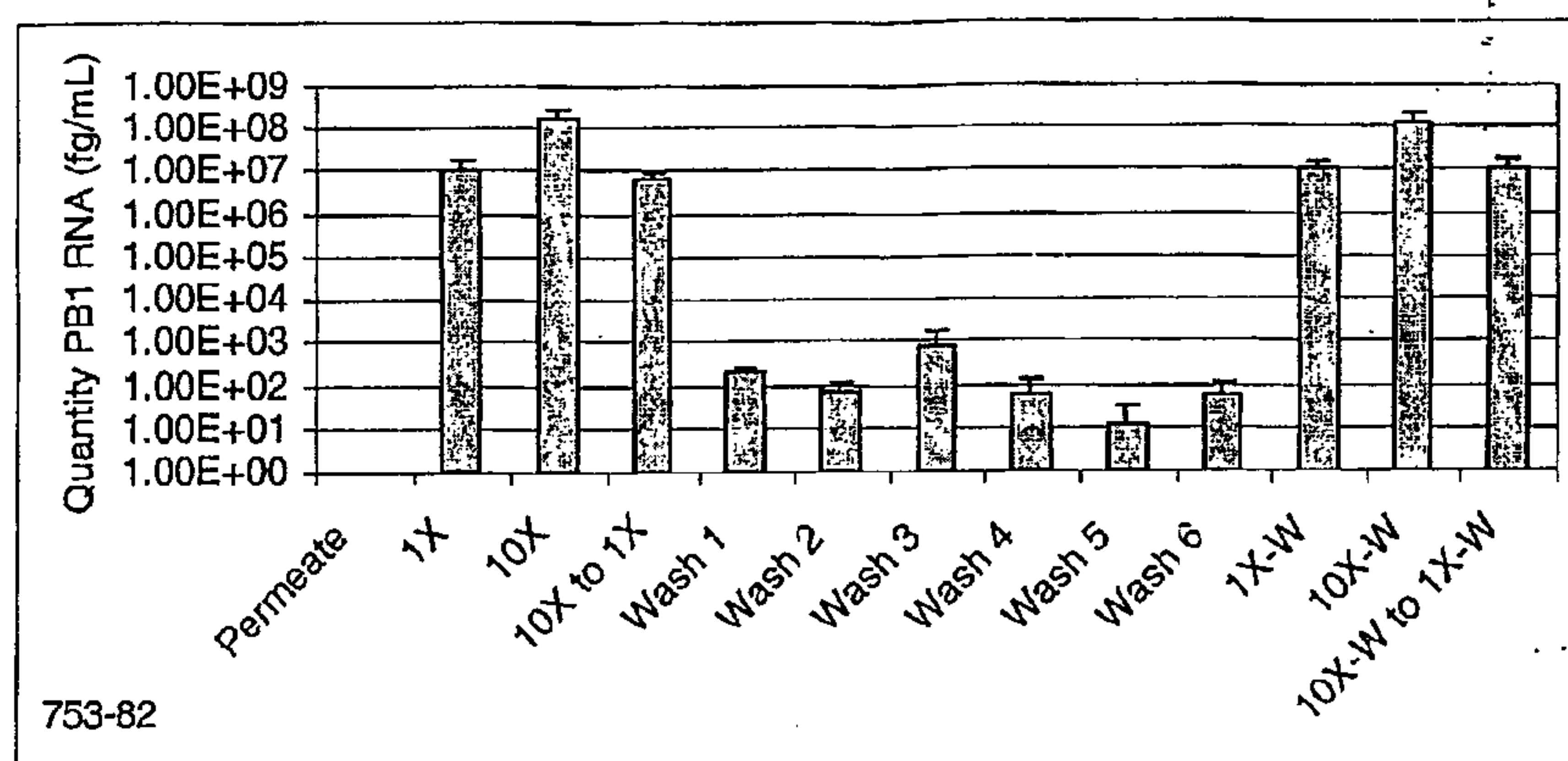
Figure 33: RNA analysis by RTPCR
