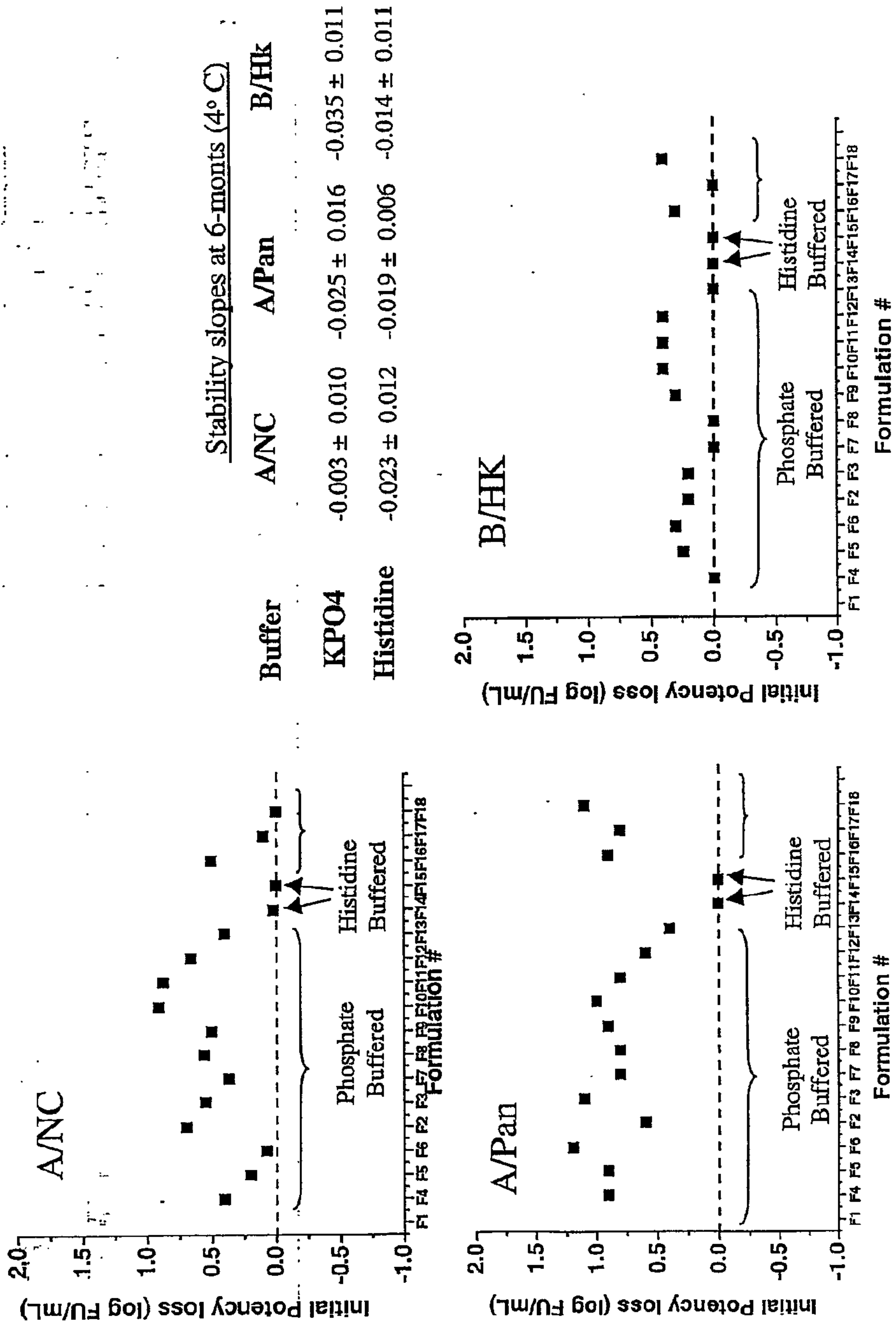
Figure 44: Initial potency loss (Freezing and/or blending loss) exclusively associated with phosphate buffered formulations
