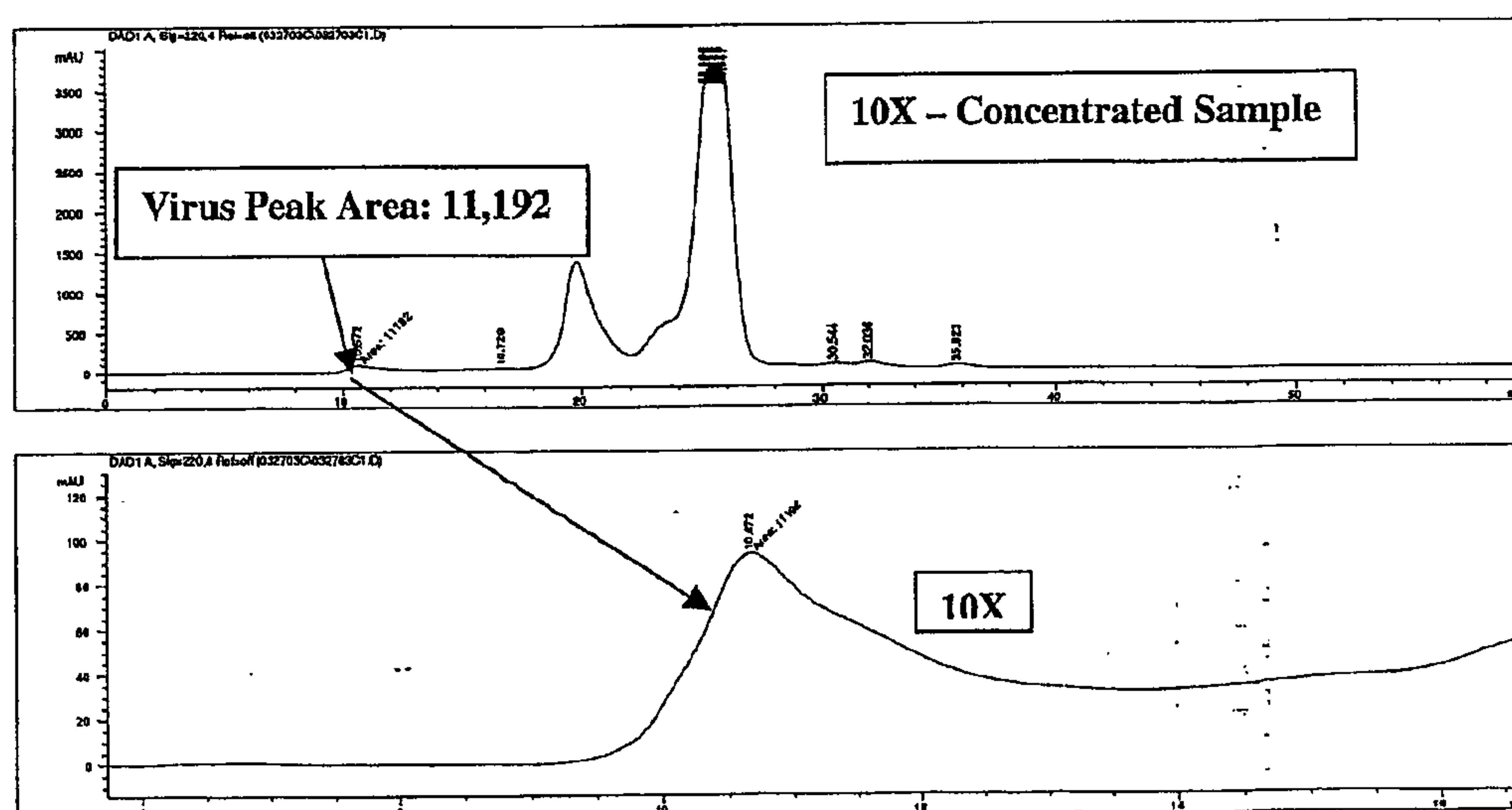
A/New Caledonia/20/99, 10X Concentrated Sample
