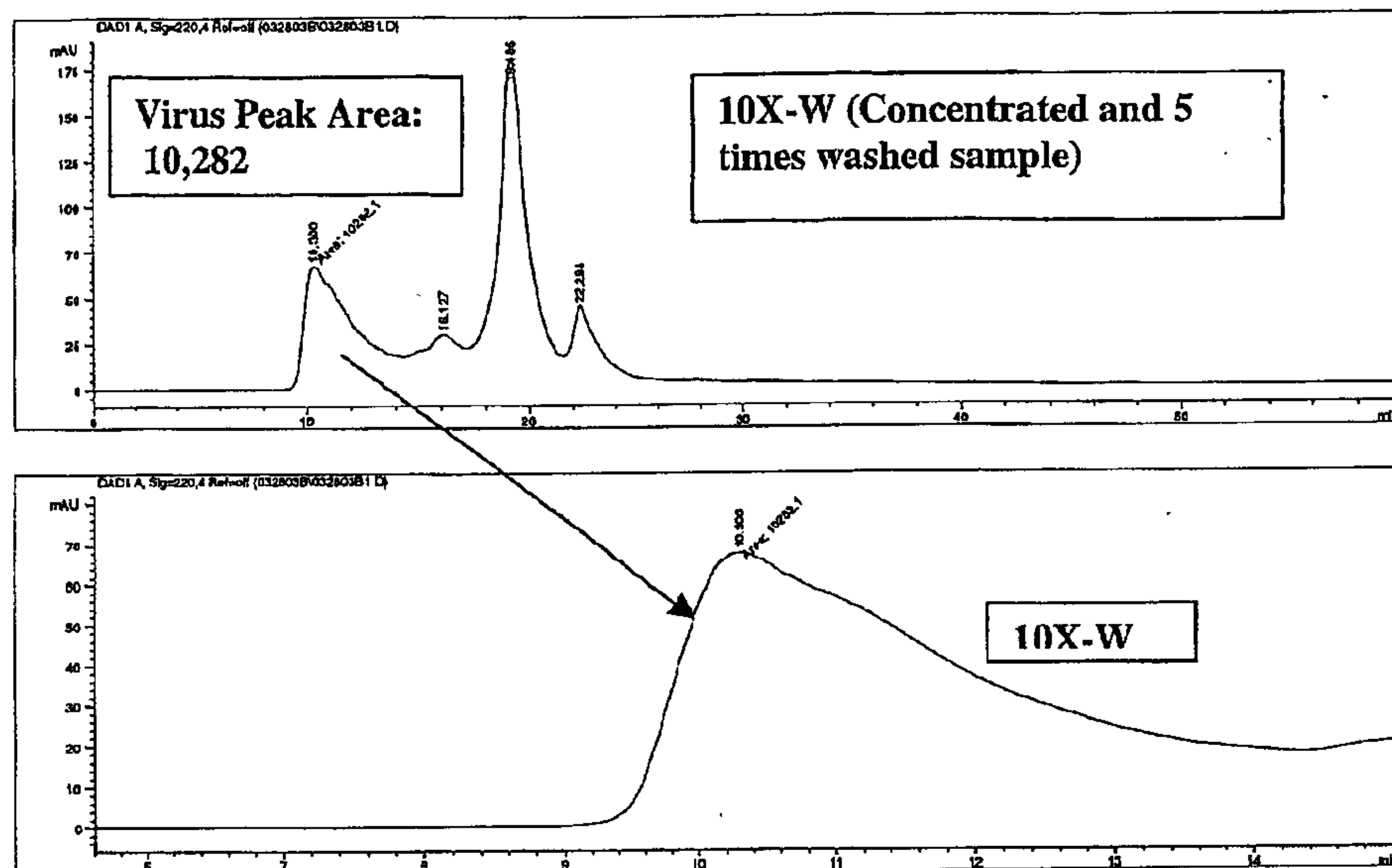
Figure 32: A/New Caledonia/20/99- 10X-W, Sample after 5 washes
