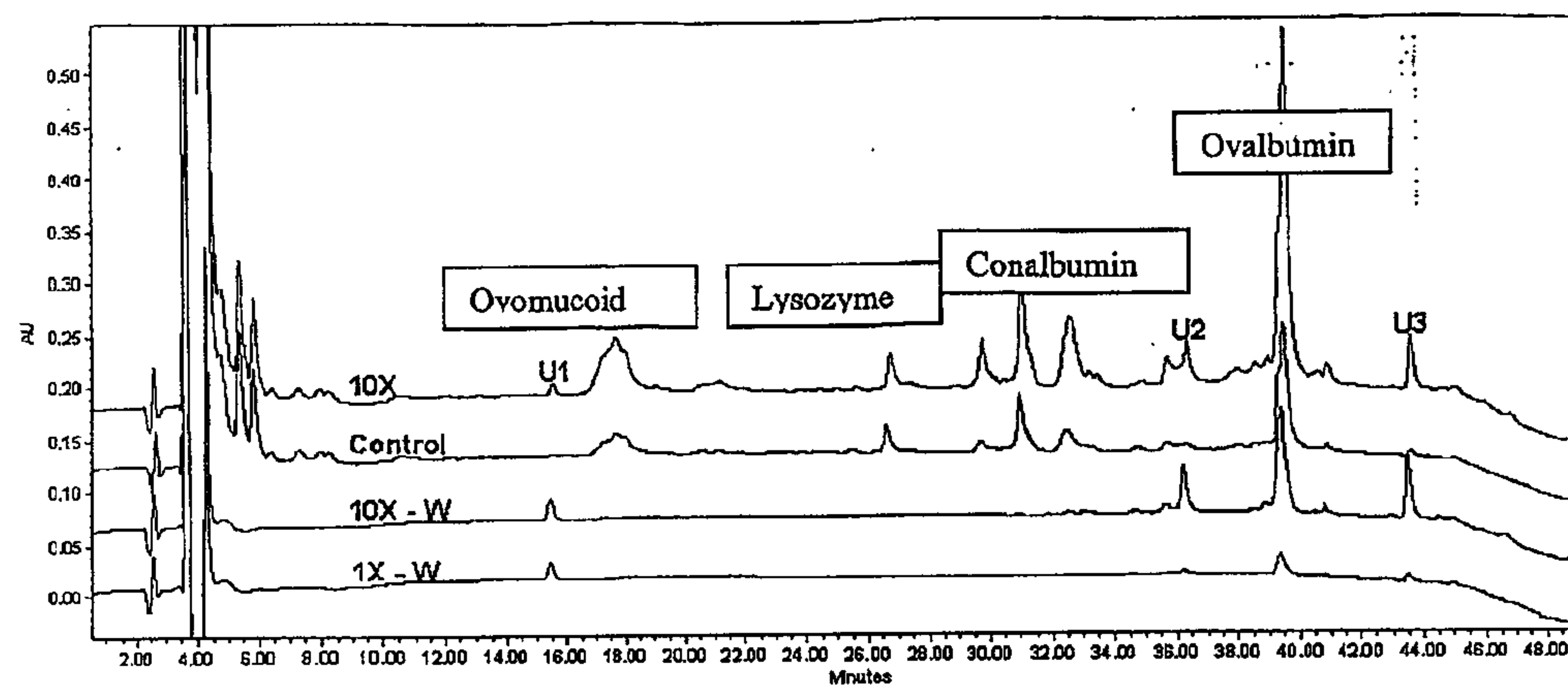
Figure 23: RHPLC of Control, 10X, 10X-W, and 1X-W
