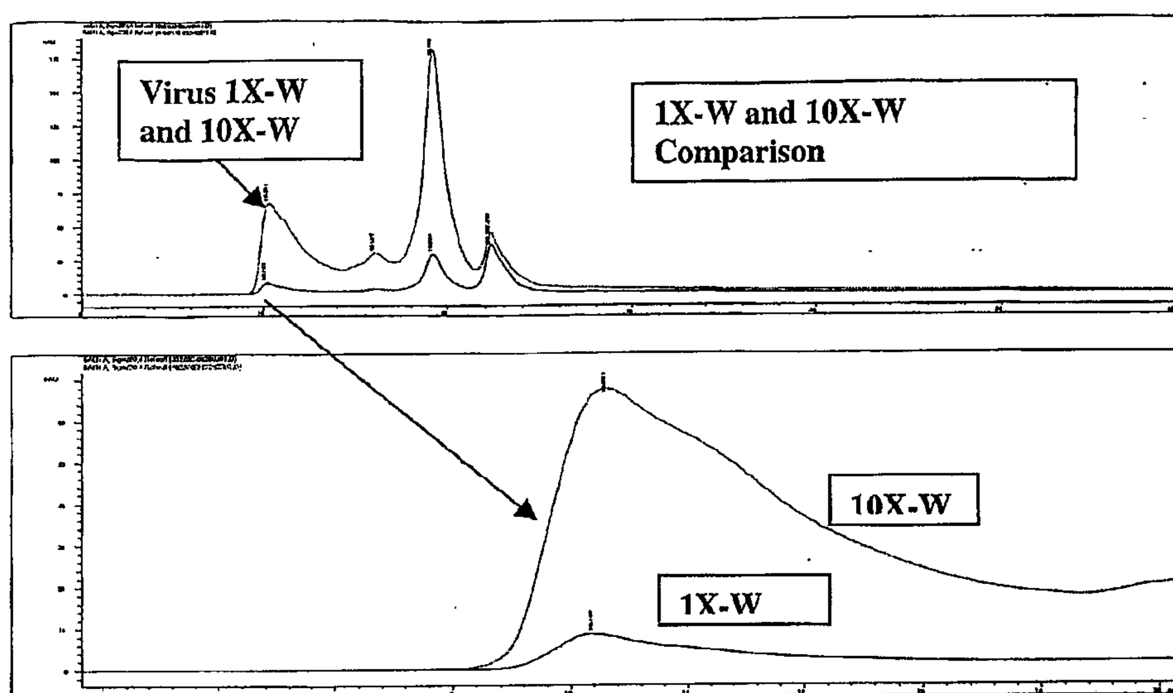
Figure 20: A/New Caledonia/20/99 – 1XW and 10X-W, Comparison
