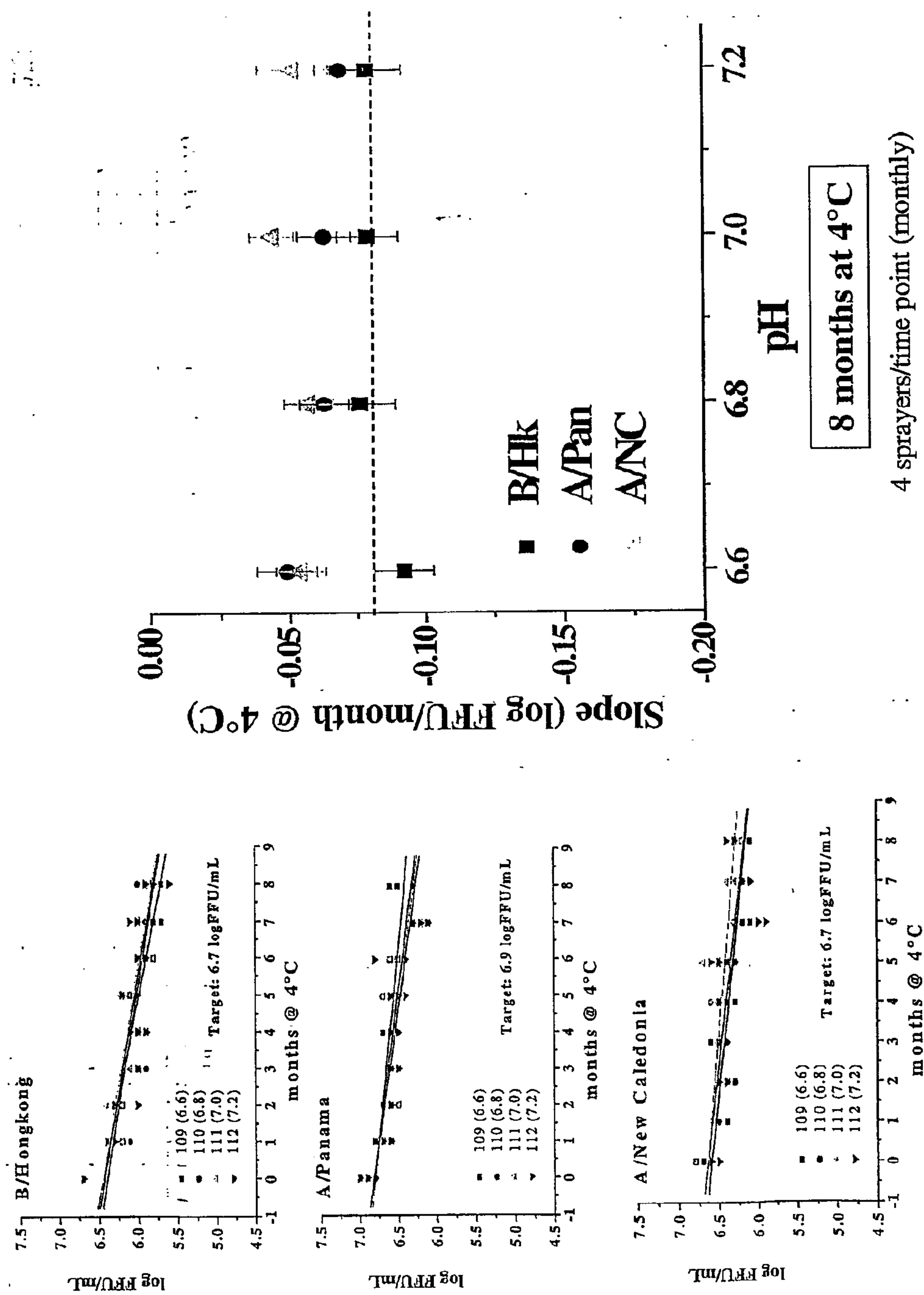
Figure 48: Optimal pH of Histidine-based 10/2/2 formulation
