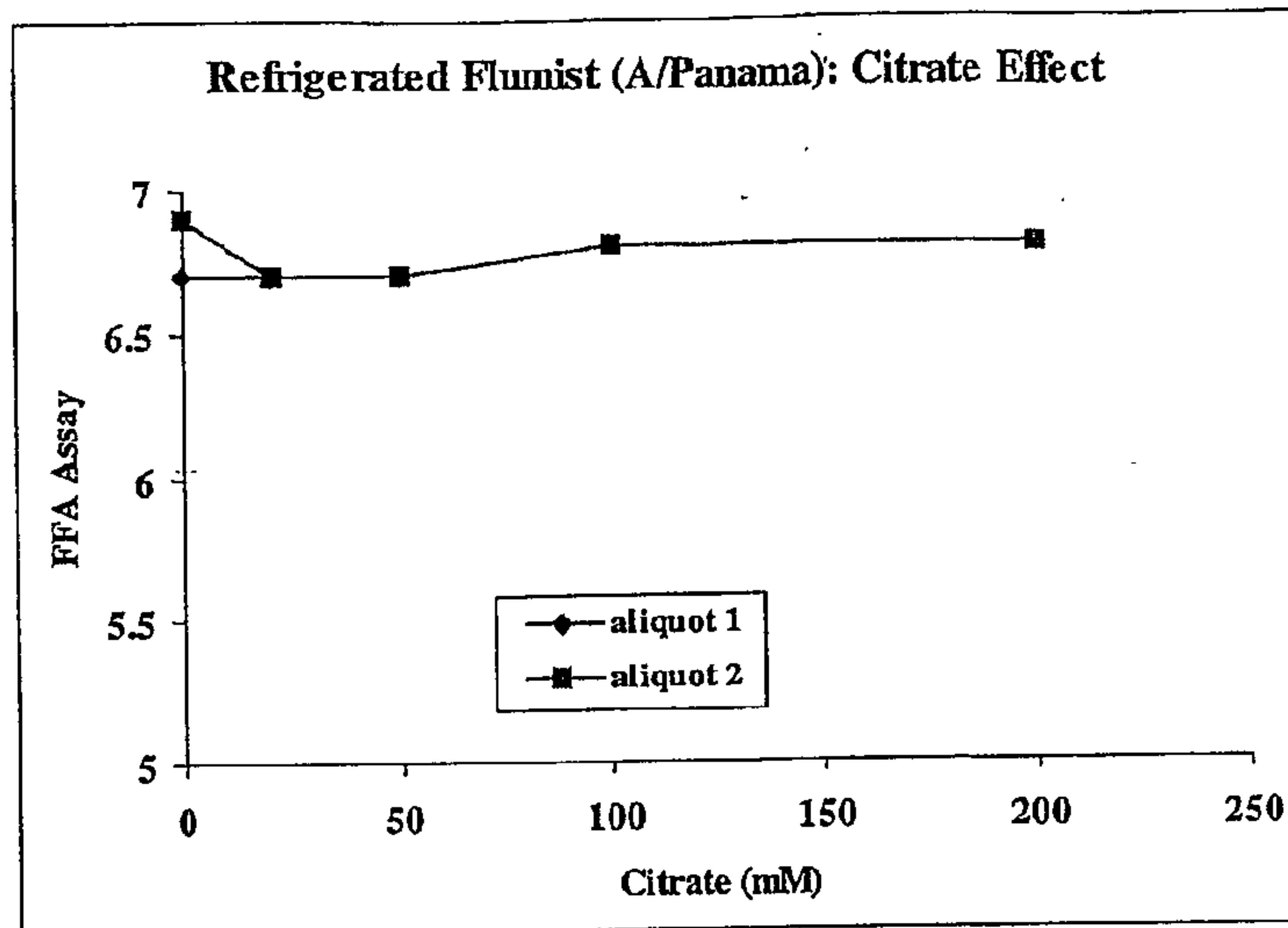
Figure 41 a-c: Base Formulation: 60% NAF, 10% Sucrose, 1% Gelatin 2% Arginine
