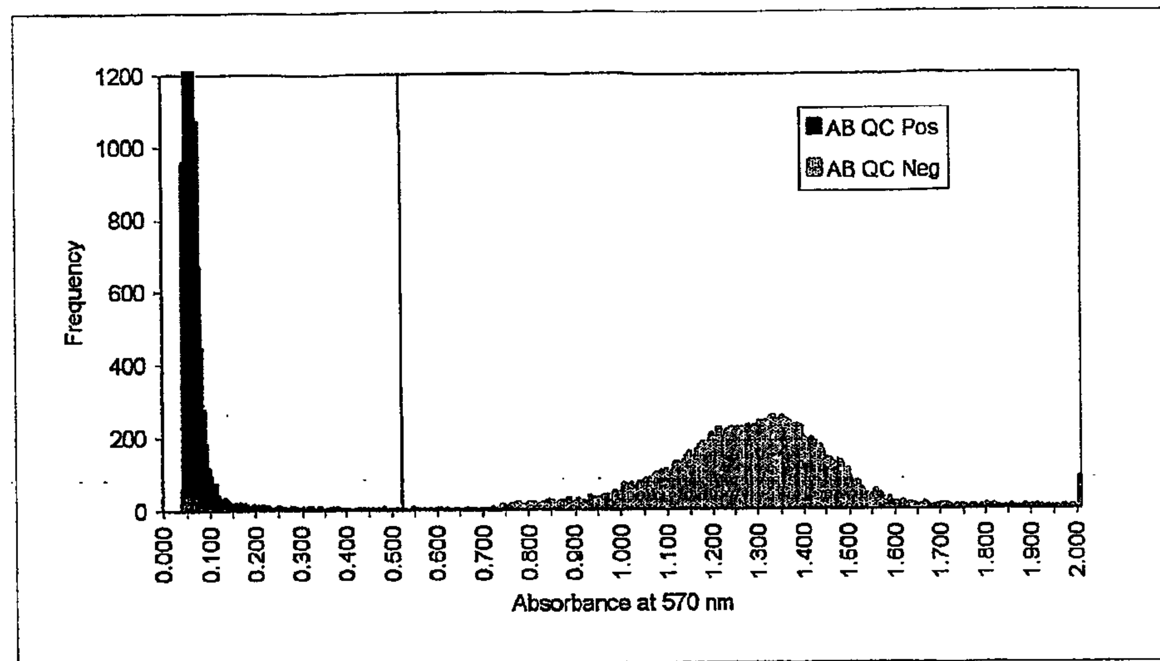
Figure50: Histogram of Absorbance at 570 nm Versus the Frequency of Occurrence
