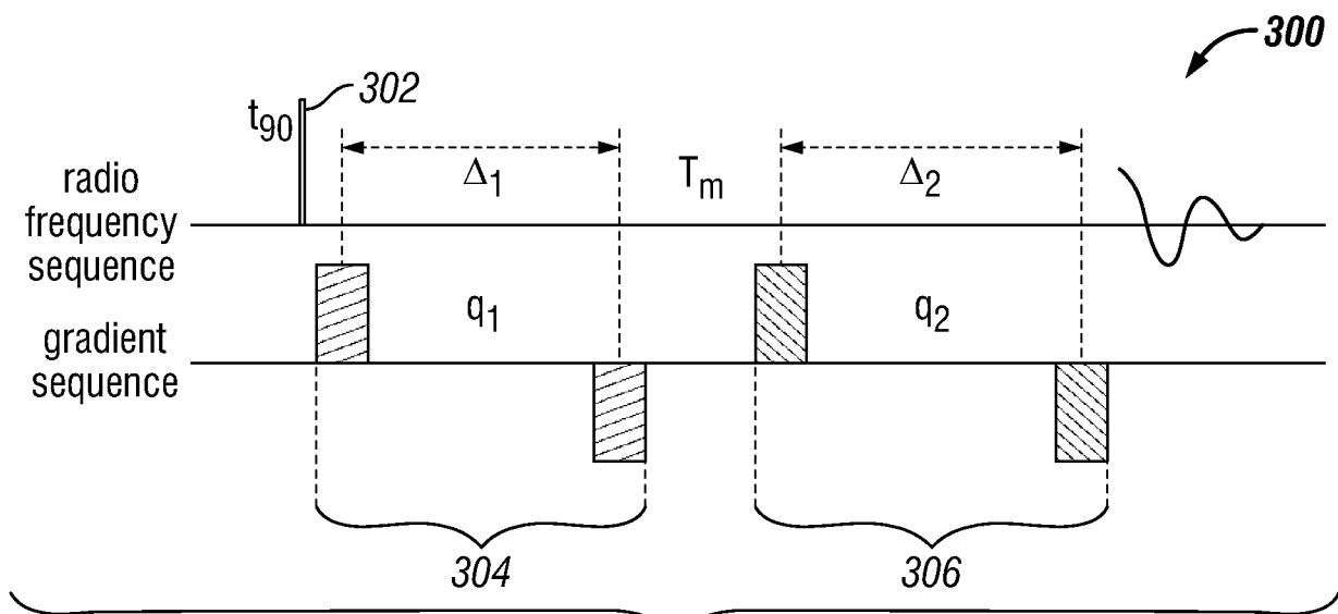
FIG. 3 (Prior Art)
