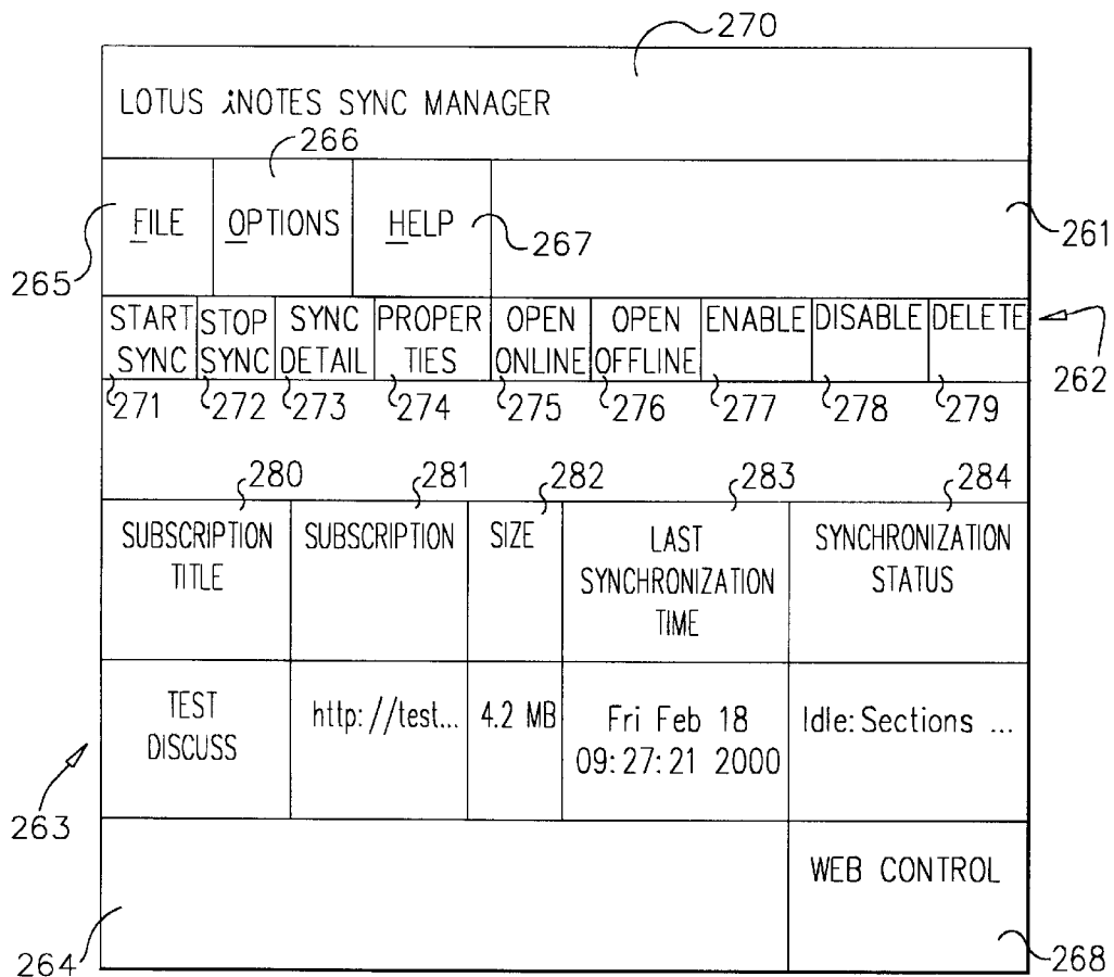
LOTUS iNOTES SYNC MANAGER INITIAL WINDOW
