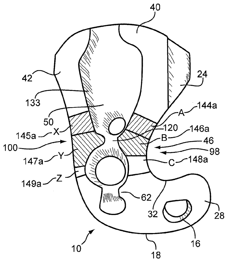
FIG. 16 PRIOR ART
