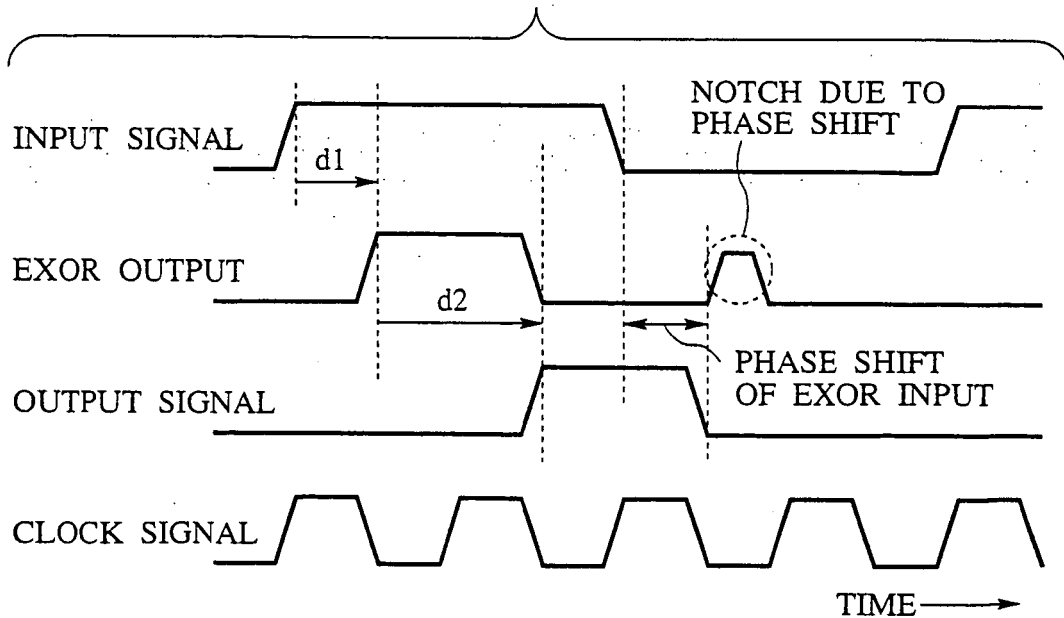
FIG.4 PRIOR ART
