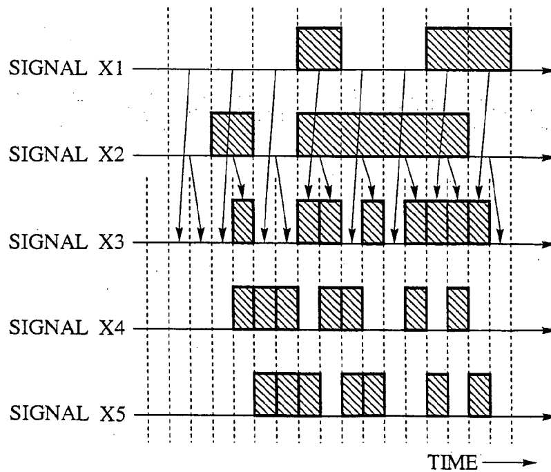
FIG.2 PRIOR ART
