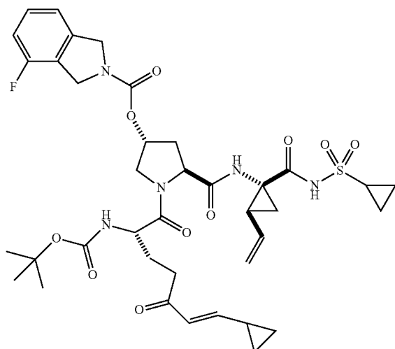
I-77
