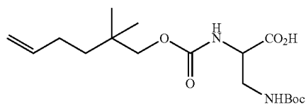
Intermediate 9-2
