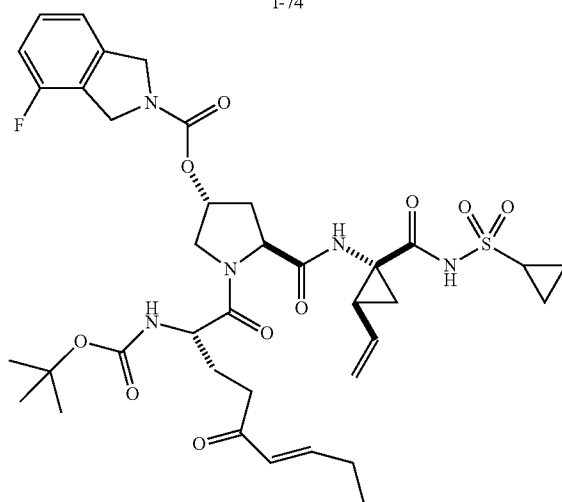
I-75
