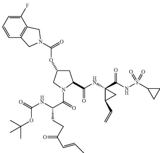
I-26
