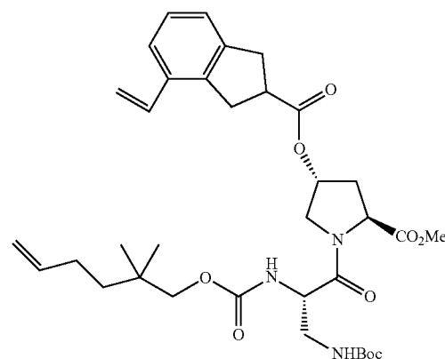
Intermediate 9-5
