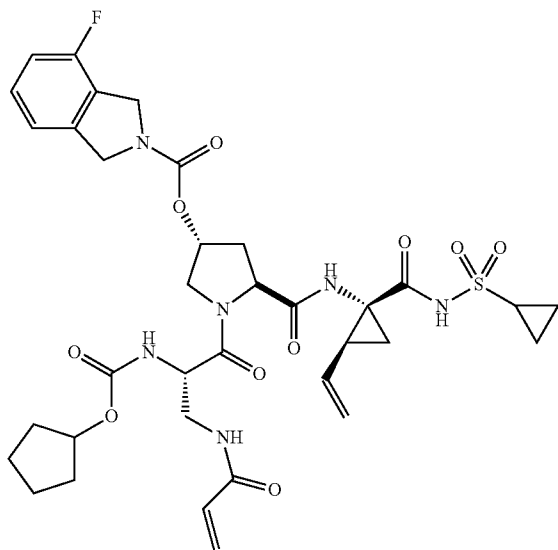
I-19
