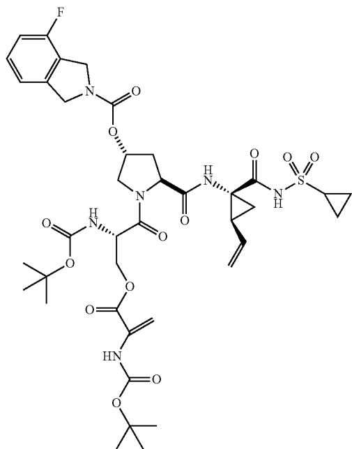
(3R,5S)-1-((S)-2-(tert-butoxycarbonylamino)-3-(2-(tert-butoxycarbonylamino)acryloyloxy)propanoyl)-5-((1R,2S)-1-(cyclopropylsulfonylcarbamoyl)-2-vinylcyclopropylcarbamoyl)pyrrolidin-3-yl-4-fluoroisoindoline-2-carboxylate
