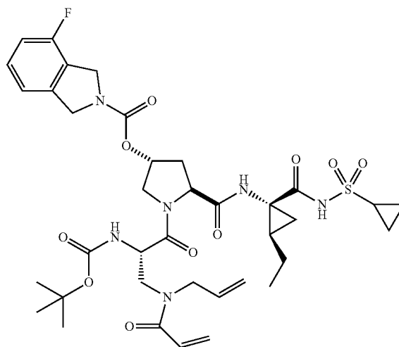
(3R,5S)-1-(S)-3-(N-allylacrylamido)-2-(tert-butoxycarbonylamino)propanoyl)-5-((1R,2R)-1-(cyclopropylsulfonylcarbamoyl)-2-ethylcyclopropylcarbamoyl)pyrrolidin-3-yl-4-fluoroisindoline-2-carboxylate
