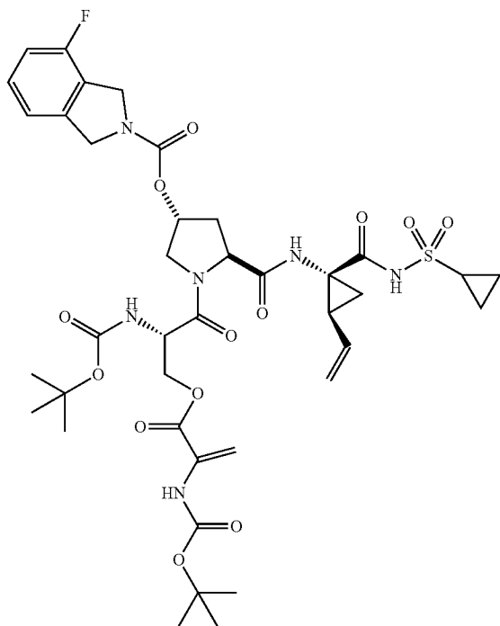
I-23
