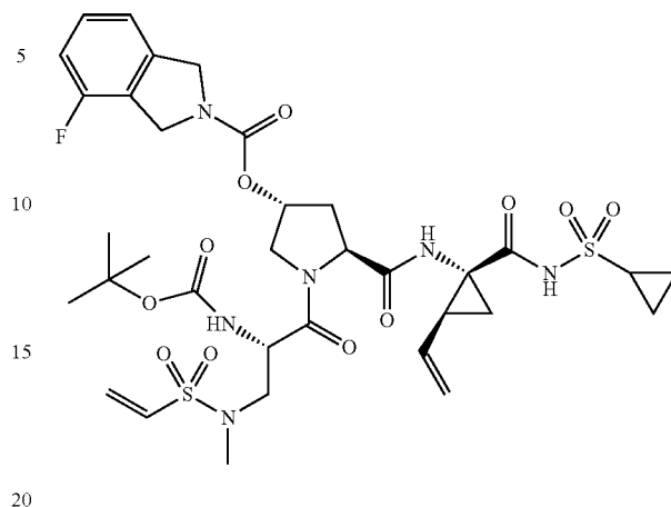
(3R,5S)-1-((S)-2-(tert-butoxycarbonylamino)-3-(N-methylvinylsulfonamido)propanoyl)-5-((1R,2S)-1-(cyclopropylsulfonylcarbamoyl)-2-vinylcyclopropylcarbamoyl)pyrrolidin-3-yl 4-fluoroisindoline-2-carboxylate
