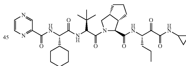
VX-950
