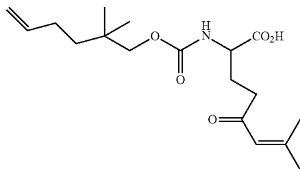
Intermediate 10-2
