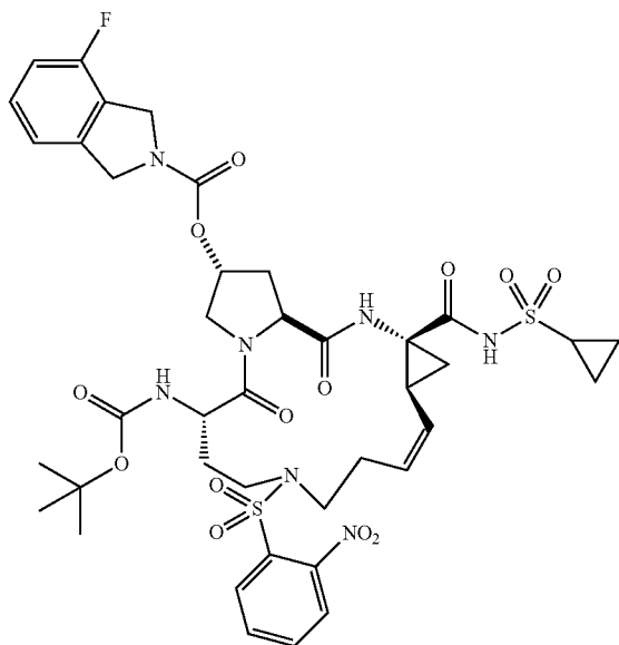
I-53
