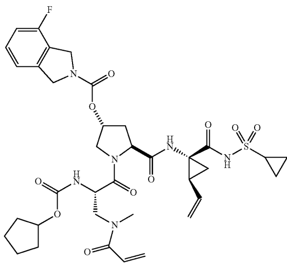
I-20
