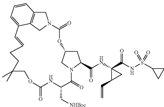
Macrocycle Intermediate 9-8
