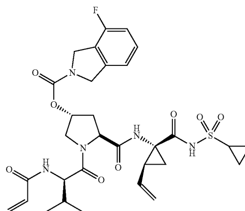
(3R,5S)-1-((R)-2-acrylamido-3-methylbutanoyl)-5-((1R,2S)-1-(cyclopropylsulfonylcarbamoyl)-2-vinylcyclopropylcarbamoyl)pyrrolidin-3-yl-4-fluoroisindoline-2-carboxylate
