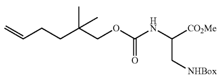
Intermediate 9-1
