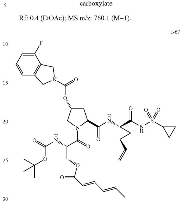
(3R,5S)-1-((S)-2-(tert-butoxycarbonylamino)-3-(2E,4E)-hexa-2,4-dienoyloxy)propanoyl)-5-((1R,2S)-1-(cyclopropylsulfonylcarbamoyl)-2-vinylcyclopropylcarbamoyl)pyrrolidin-3-yl-4-fluoroisoindoline-2-carboxylate
