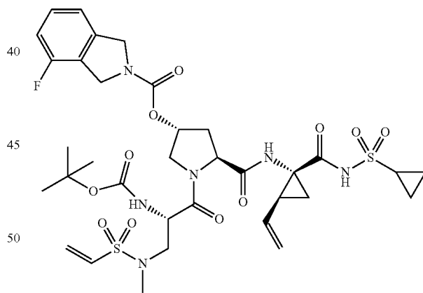
(3R,5S)-1-(S)-2-(tert-butoxycarbonylamino)-4-(N-methylacrylamido)butanoyl-5-((1R,2S)-1-(cyclopropylsulfonylcarbamoyl)-2-vinylcyclopropylcarbamoyl)pyrrolidin-3-yl 4-fluoroisindoline-2-carboxylate
