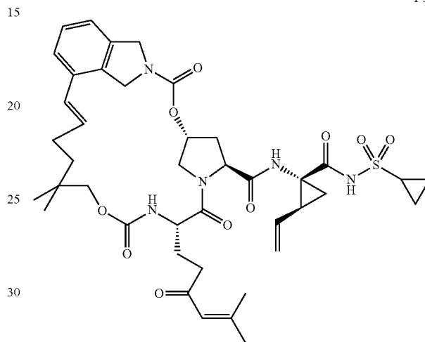
Intermediate 10-2
