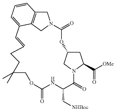
Macrocytic Intermediate 9-6
