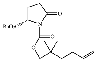
Intermediate 10-1
