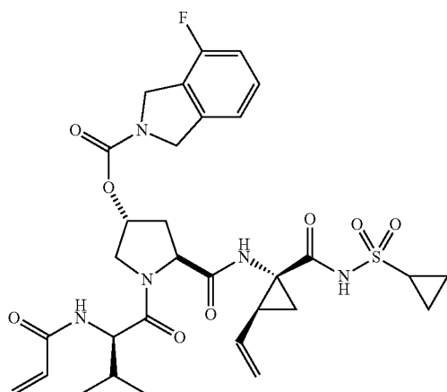
I-9
