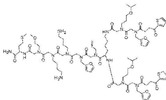
Chemical Formula: C_{66}H_{127}N_{19}O_{21}S_3 Molecular Weight: 1603.23
