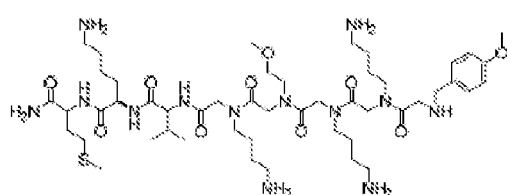
Chemical Formula: C_{42}H_{52}N_{11}O_{10}S Molecular Weight: 1052.39
