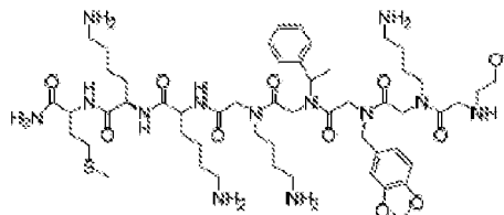
Chemical Formula: C_{54}H_{62}N_{13}O_{11}S Molecular Weight: 1128.45
