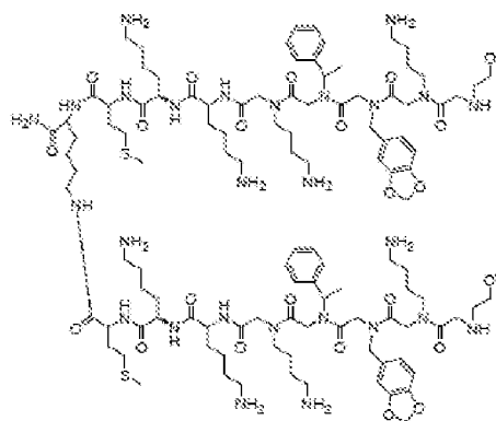
Chemical Formula: C_{114}H_{197}N_{27}O_{31}S_5 Molecular Weight: 2305.04
