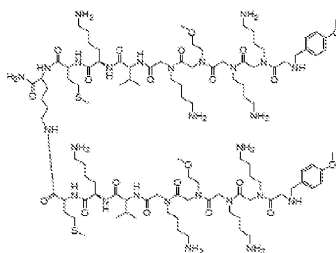
Chemical Formula: C_{104}H_{187}N_{27}O_{31}S_5 Molecular Weight: 2215.83
