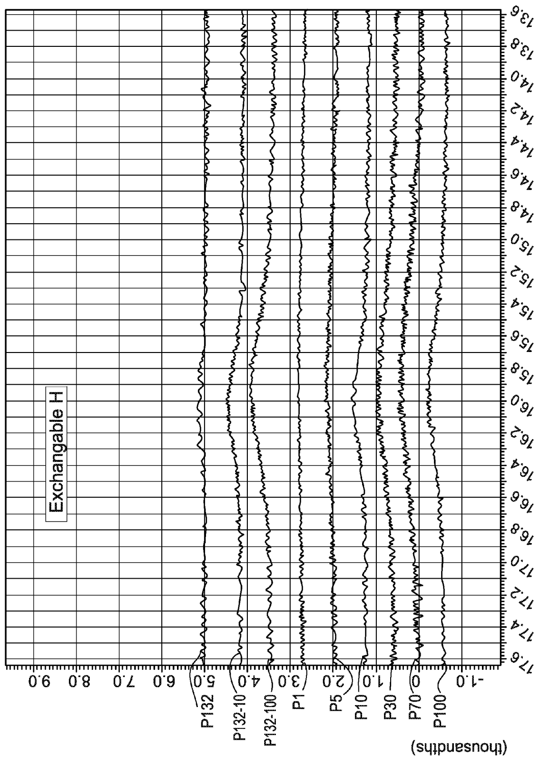
FIG. 38J X : parts per Million : ^1\text{H}
