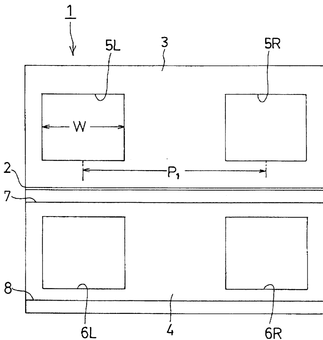
FIG 12 (PRIOR ART)
