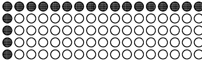
Prediction mode 2
