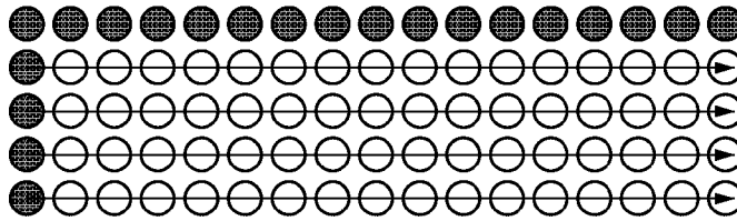
Prediction mode 1
