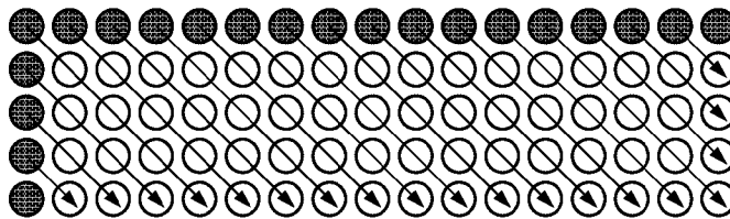
Prediction mode 4
