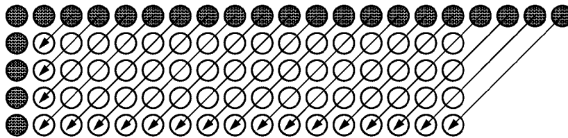
Prediction mode 3
