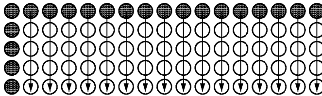
Prediction mode 0
