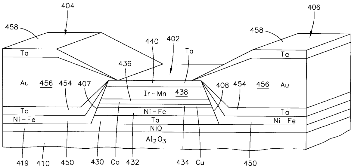
(AFM STABILIZATION)
