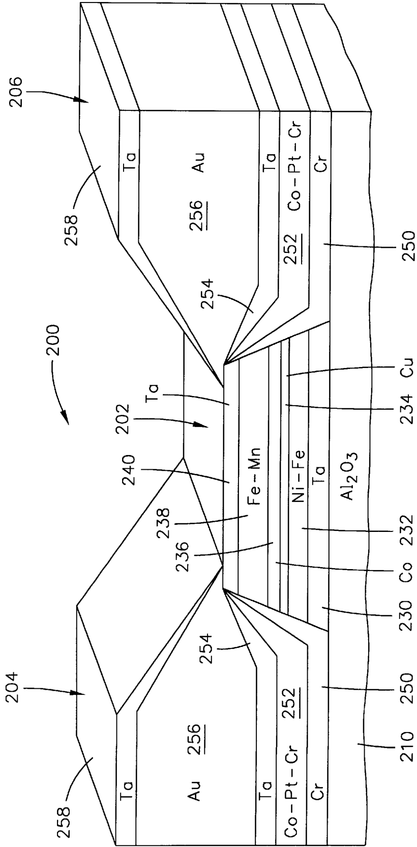
FIG. 11 (HM STABILIZATION)
