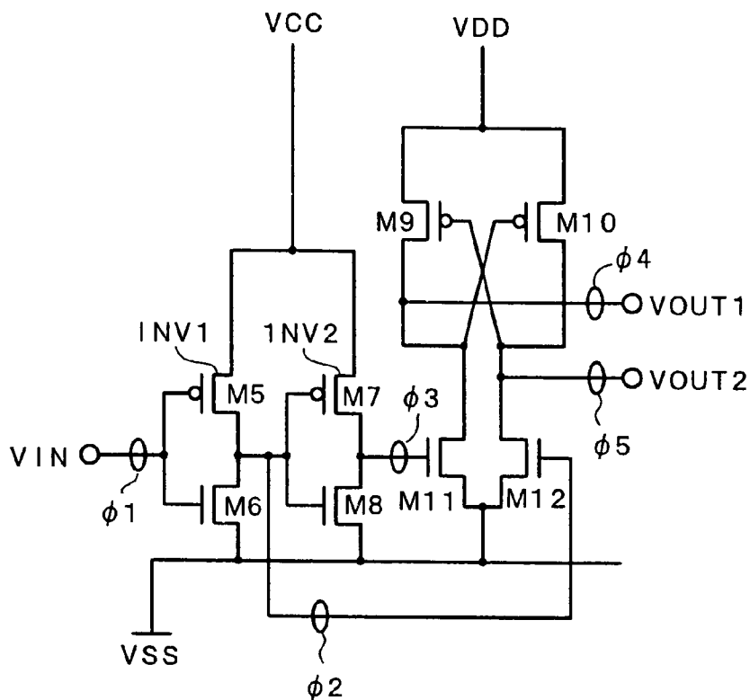
FIG. 14 (PRIOR ART)
