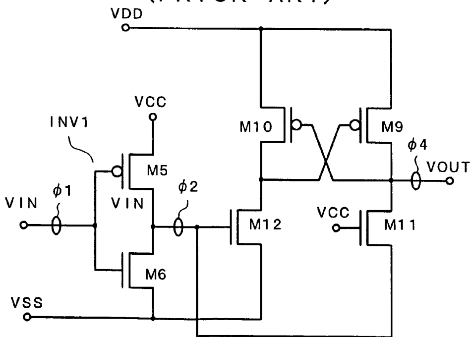
FIG. 14 (PRIOR ART)
