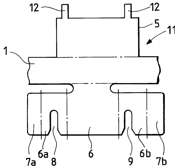
FIG. 9 PRIOR ART
