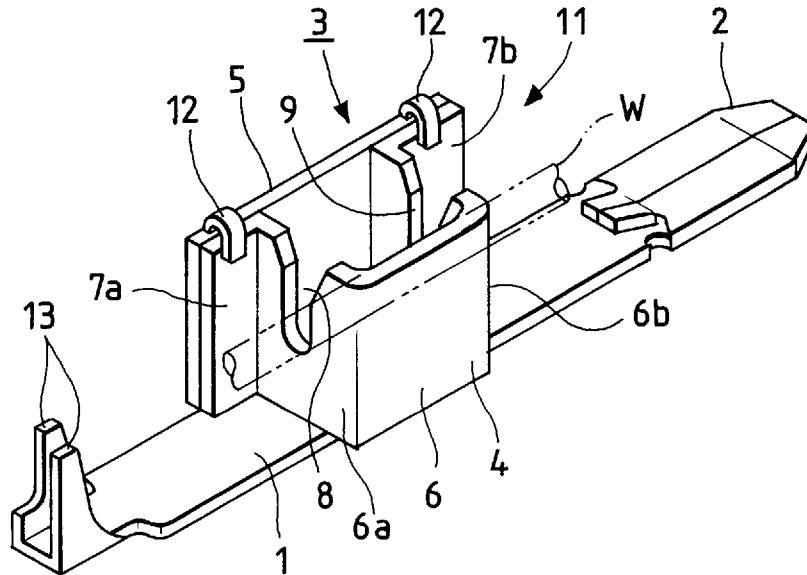
FIG. 8 PRIOR ART
