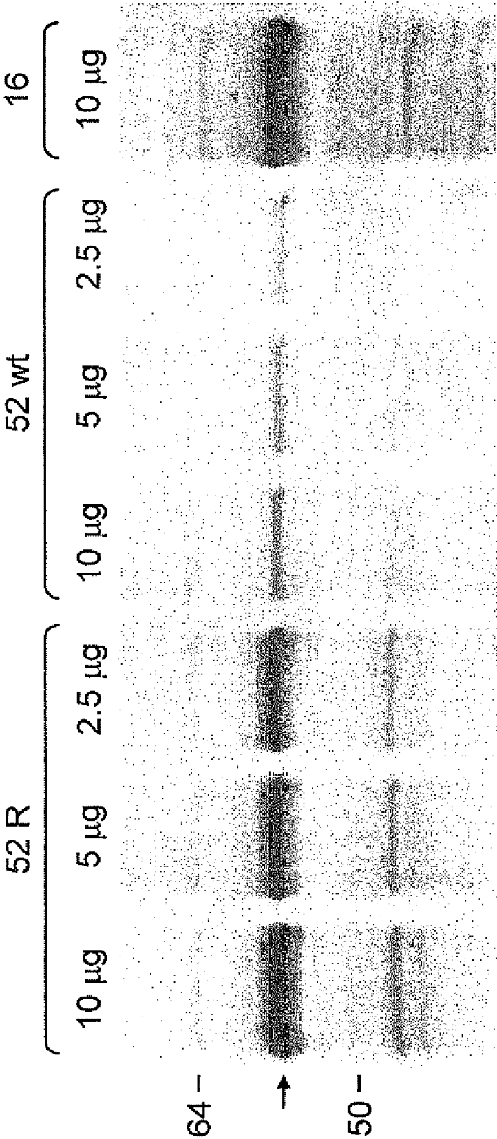
Western Blot Analysis of HPV 52 L1 Protein
