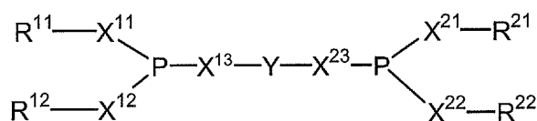
Formula (III)
