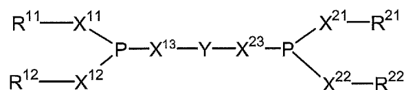
Formula (III)
