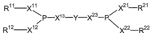
Formula (III)
