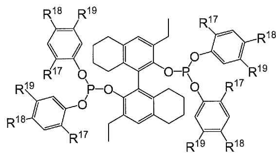
(IX)
