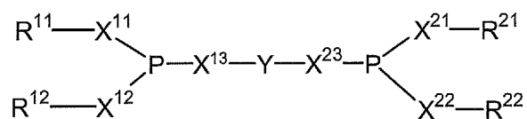
Formula (III)
