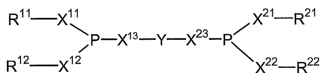
Formula (III)
