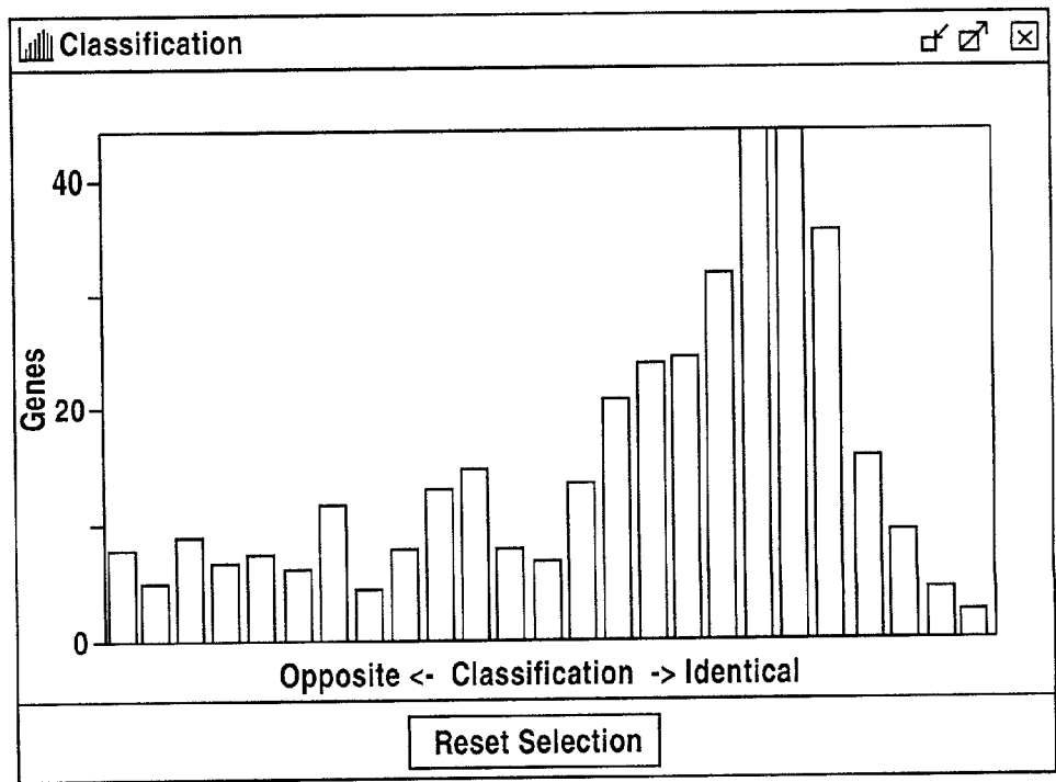
The Classification histogram created using the "adjust scales" scaling procedure and the data displayed in the "Classify Experiments" dialog box above (Figure 41).
