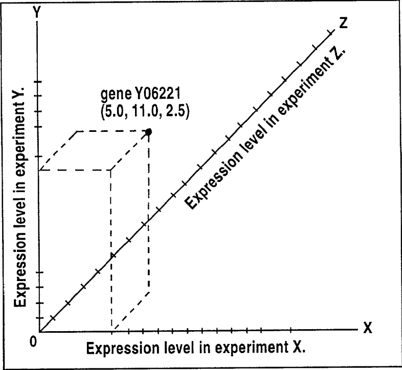
A point (gene) plotted in three dimensions.
