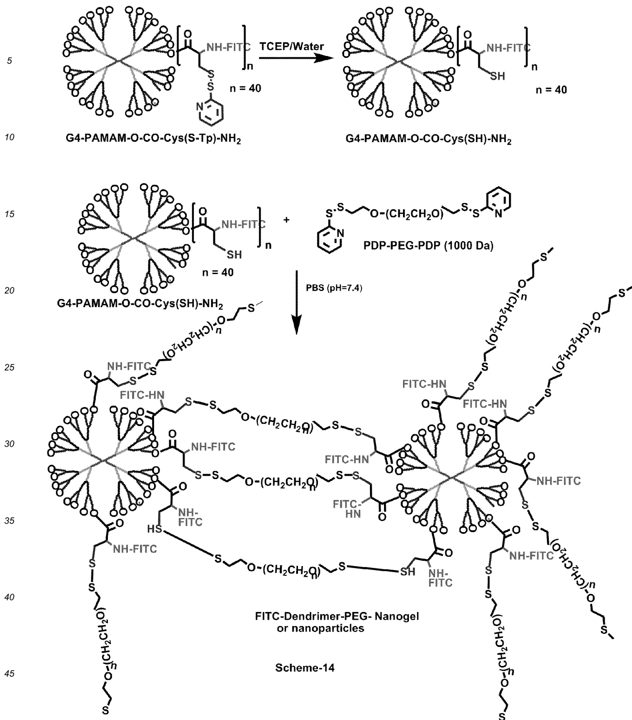
[0146] Scheme-14: G4-O-CO-Cys(SH)-NH 2 cross linked with PDP-PEG-PDP to form dendrimer-PEG nanogel (or nanoparticles)
