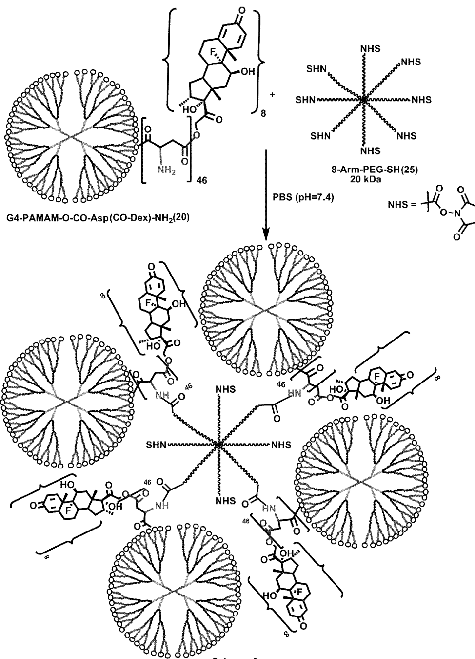
Scheme-6 G4-PAMAM-O-CO-Asp(CO-Dex)-NH 2 -PEG Hydrogel (26)
