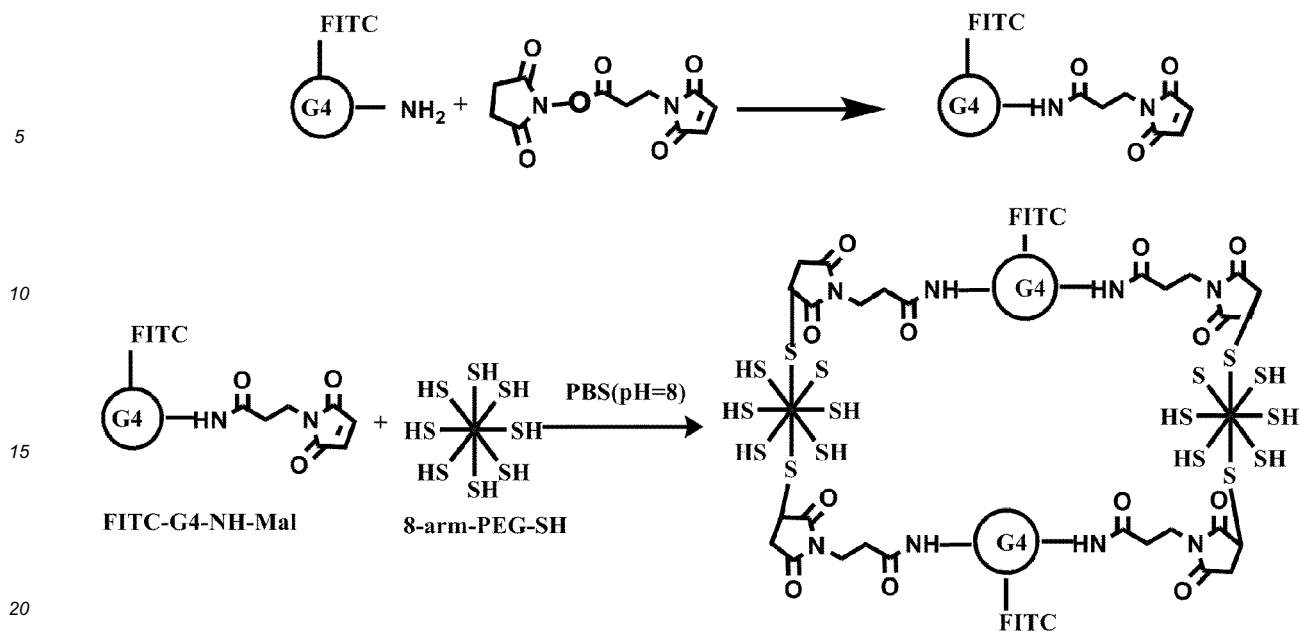
Scheme-12 Dendrimer-FITC Covalently linked Dendrimer -PEG nanogel or Particles
