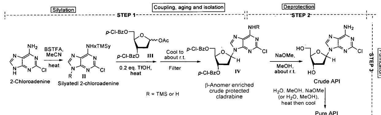
Scheme 7 - synthesis of cladribine in accordance with a preferred embodiment of the present application
