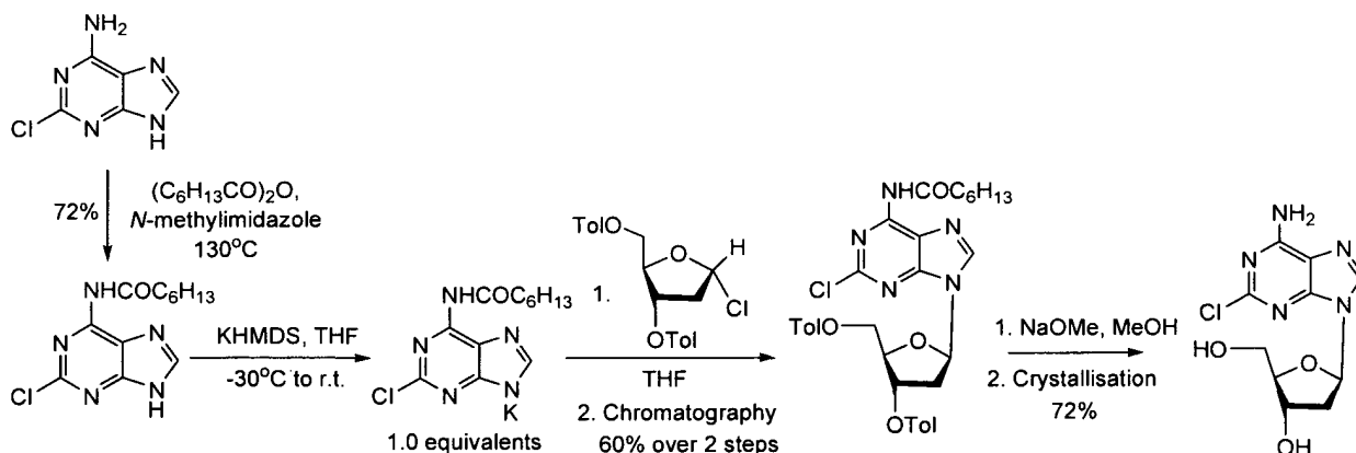
Scheme 5- Gupta and Munk's cladribine synthesis
