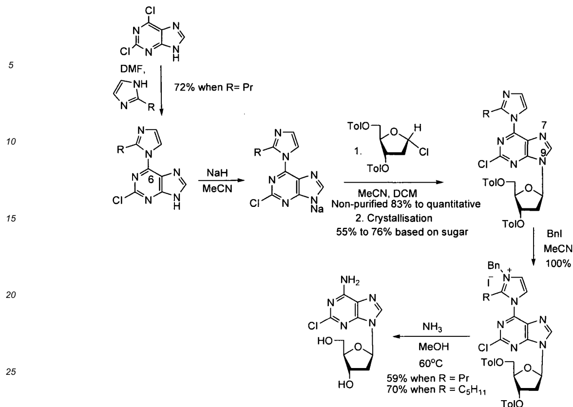
Scheme 6-Robins' 6-(imidazol-1-yl)-based cladribine synthesis
