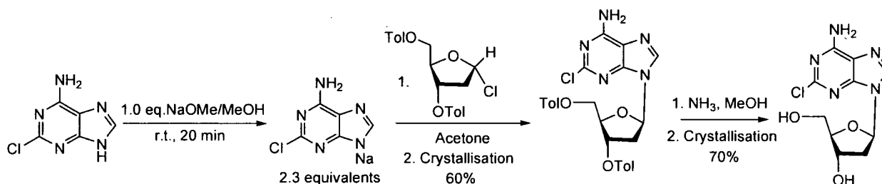
Scheme 4- Gerszberg and Alonso's cladribine synthesis
