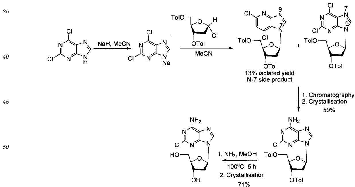
Scheme 3-Robins' S_N2 Approach
