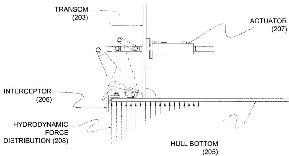
FIGURE-2 CONVENTIONAL 1-DOF INTERCEPTOR (206)
