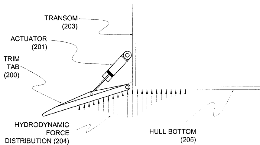
FIGURE-1 CONVENTIONAL 1-DOF TRIM-TAB (200)
