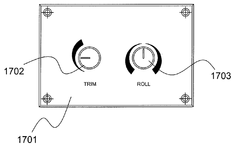
FIGURE-17B, INDIVIDUAL TRIM & ROLL CONTROL KNOBS, ABSOLUTE ADJUSTMENT METHOD (514)
