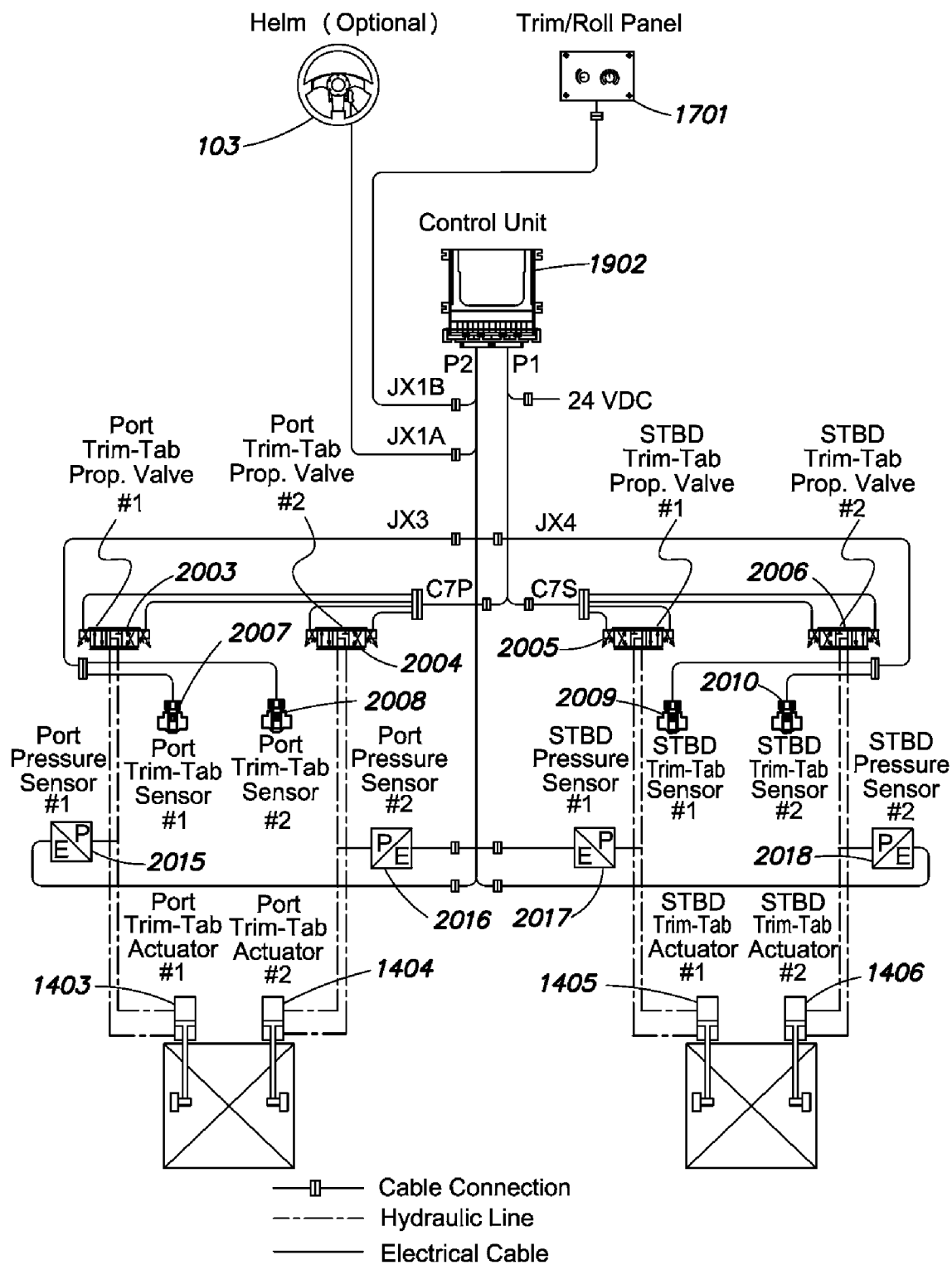
FIGURE 20 SYSTEM DIAGRAM 1DOF TRIM-TAB INTEGRATED WITH WATERJETS
