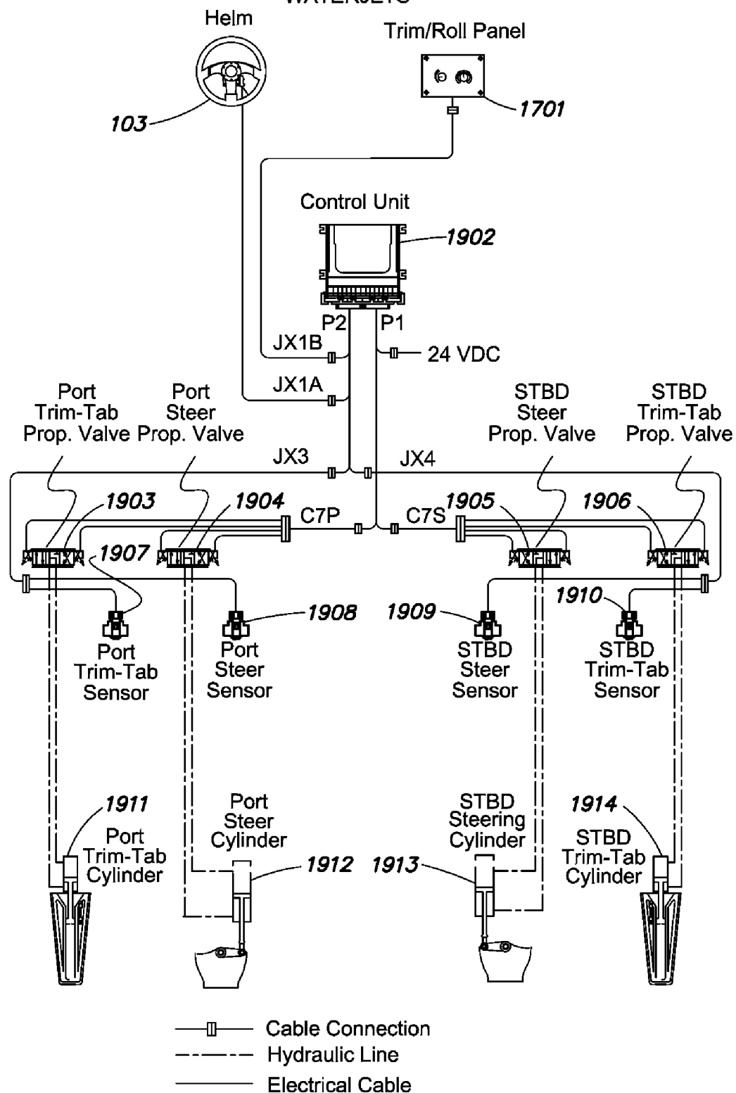
FIGURE 19 SYSTEM DIAGRAM 1DOF TRIM-TAB INTEGRATED WITH WATERJETS
