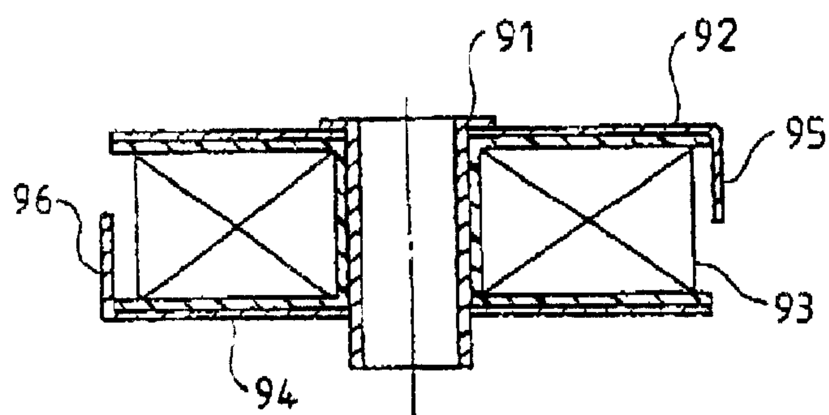
FIG.12 PRIOR ART
