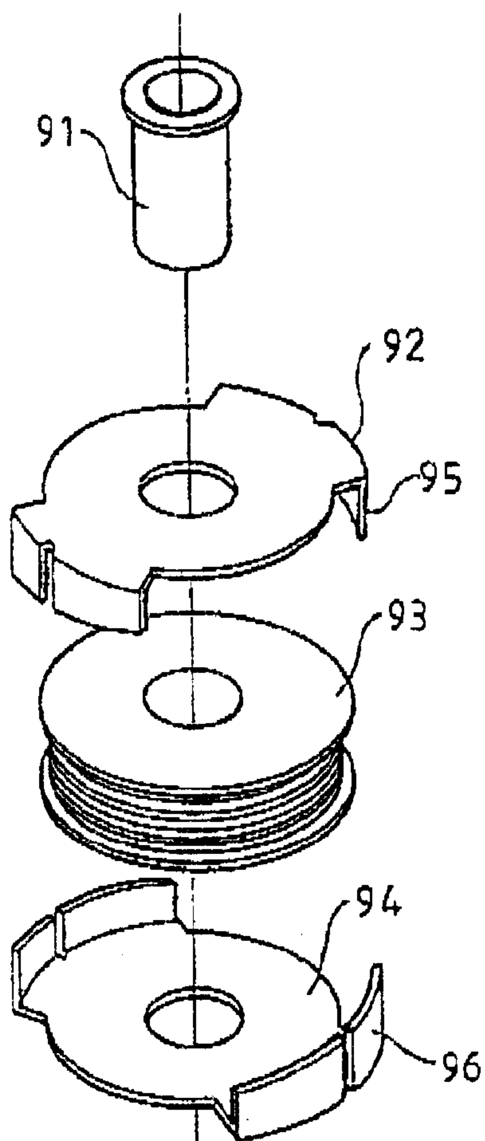
FIG.11 PRIOR ART
