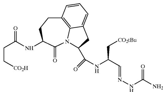
(2S-cis)-[5-succinylamino-1,2,3,4,5,6,7-hexahydro-4-oxoazepino[3,2,1-hi]Indole-2-carbonyl)-amino]-4-oxo-butanoic Acid Tert-butyl Ester Semicarbazone
