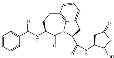
(2S-cis)-[5-benzoylamino-1,2,3,4,5,6,7-hexahydro-4-oxoazepino[3,2,1-hi][indole-2-carbonyl]-amino]-4-oxo-butanoic Acid Semicarbazone
