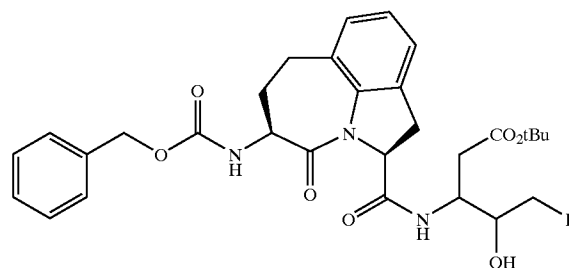
3-((2S-cis)-[5-benzyloxycarbonylamino-1,2,3,4,5,6,7-hexahydro-4-oxoazepino[3,2,1-hi]indole-2-carbonyl)-amino]-5-fluoro-4-hydroxy-pentanoic Acid Tert-butyl Ester
