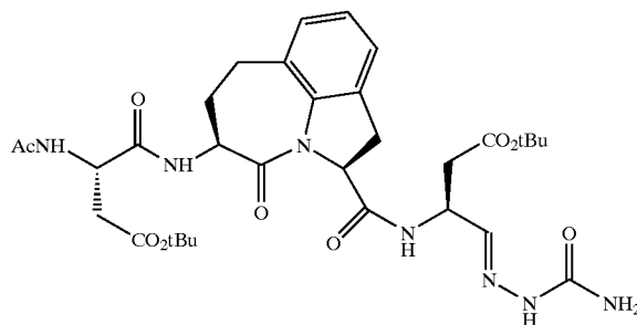
(2S-cis)-[5-(N-acetyl-(S)-aspartyl- \beta -tert-butyl ester)amino-1,2,3,4,5,6,7-hexahydro-4-oxazepino[3,2,1-hi]Indole-2-carbonyl]-amino-4-oxo-butanoic Acid Tert-butyl Ester Semicarbazone
