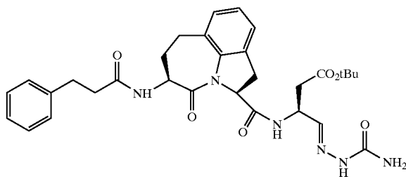
(2S-cis)-[5-(N-benzoyloxycarbonyl-(S)-aspartyl)amino-1,2,3,4,5,6,7-hexahydro-4-oxoazepino[3,2,1-hi]indole-2-carbonyl)-amino]-4-oxo-butanoic Acid Tert-butyl Ester Semicarbazone
