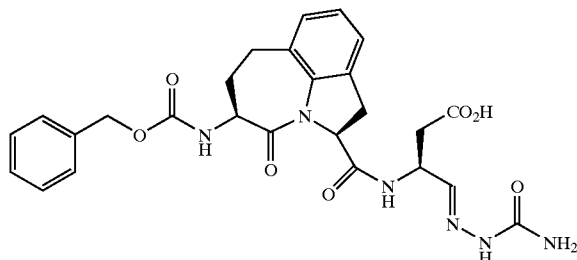
(2S-cis)-[5-benzyloxycarbonylamino-1,2,4,5,6,7-hexahydro-4-oxazepino[3,2,1-hi]indole-2-carbonyl]-amino-4-oxo-butanoic Acid Semicarbazone
