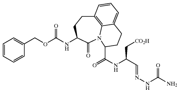
(3R,S-cis)-6-benzyloxycarbonylamino-5-oxo-2,3,4,5,6,7,8-hexahydro-1H-azepino[3,2,1-hi]quinoline-3-carbonyl)-amino]-4-oxo-butanoic Acid Tert-butyl Ester
