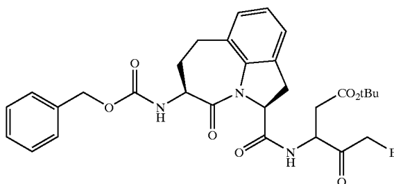
3 [(2S-cis)-[5-benzyloxycarbonylamino-1,2,3,4,5,6,7-hexahydro-4-oxoazepino[3,2,1-hi]indole-2-carbonyl)-amino]}-5-bromo-4-oxo-pentanoic Acid Tert-butyl Ester
