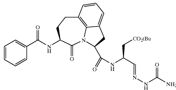
(2S-cis)-[5-benzoylamino-1,2,3,4,5,6,7-hexahydro-4-oxoazepino[3,2,1-hi]indole-2-carbonyl]-amino-4-oxo-butanoic Acid Tert-butyl Ester Semicarbazone
