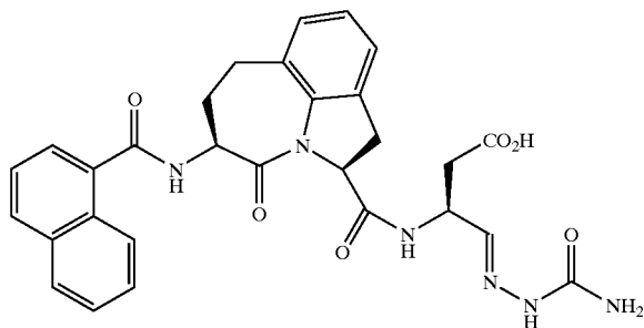
(2S-cis)-[5-(1-naphthoyl)amino-1,2,3,4,5,6,7-hexahydro-4-oxoazepino[3,2,1-hi]indole-2-carbonyl]-amino-4-oxo-butanoic Acid Semicarbazone
