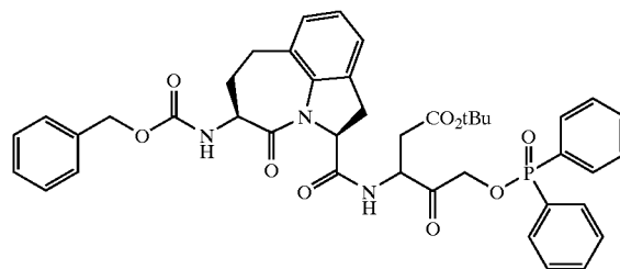
3-[(2S-cis)-[5-benzyloxycarbonylamino-1,2,3,4,5,6,7-hexahydro-4-oxoazepino[3,2,1-hi]indole-2-carbonyl]amino]-5-(diphenylphosphinyloxy)-4-oxo-pentanoic Acid Tert-butyl Ester
