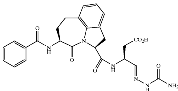
(2S-cis)-[5-benzoylamino-1,2,3,4,5,6,7-hexahydro-4-oxoazepino[3,2,1-hi][indole-2-carbonyl]-amino]-4-oxo-butanoic Acid Semicarbazone
