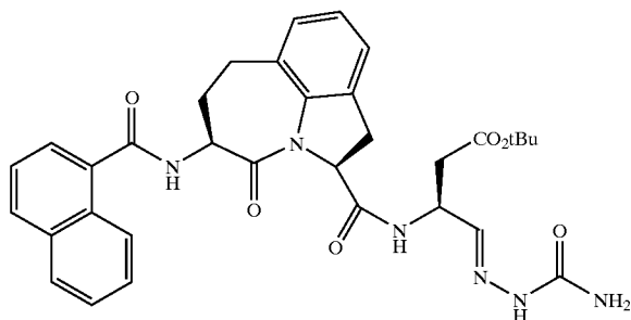
(2S-cis)-[5-(1-naphthoyl)amino-1,2,3,4,5,6,7-hexahydro-4-oxoazepino[3,2,1-hi]indole-2-carbonyl]-amino-4-oxo-butanoic Acid Tert-butyl Ester Semicarbazone
