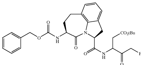
3 {(2S-cis)-[5-benzyloxycarbonylamino-1,2,3,4,5,6,7-hexahydro-4-oxoazepino[3,2,1-hi]indole-2-carbonyl)-amino]}-5-fluoro-4-oxo-pentanoic Acid Tert-butyl Ester
