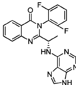
Compound C
