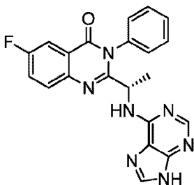
Compound B
