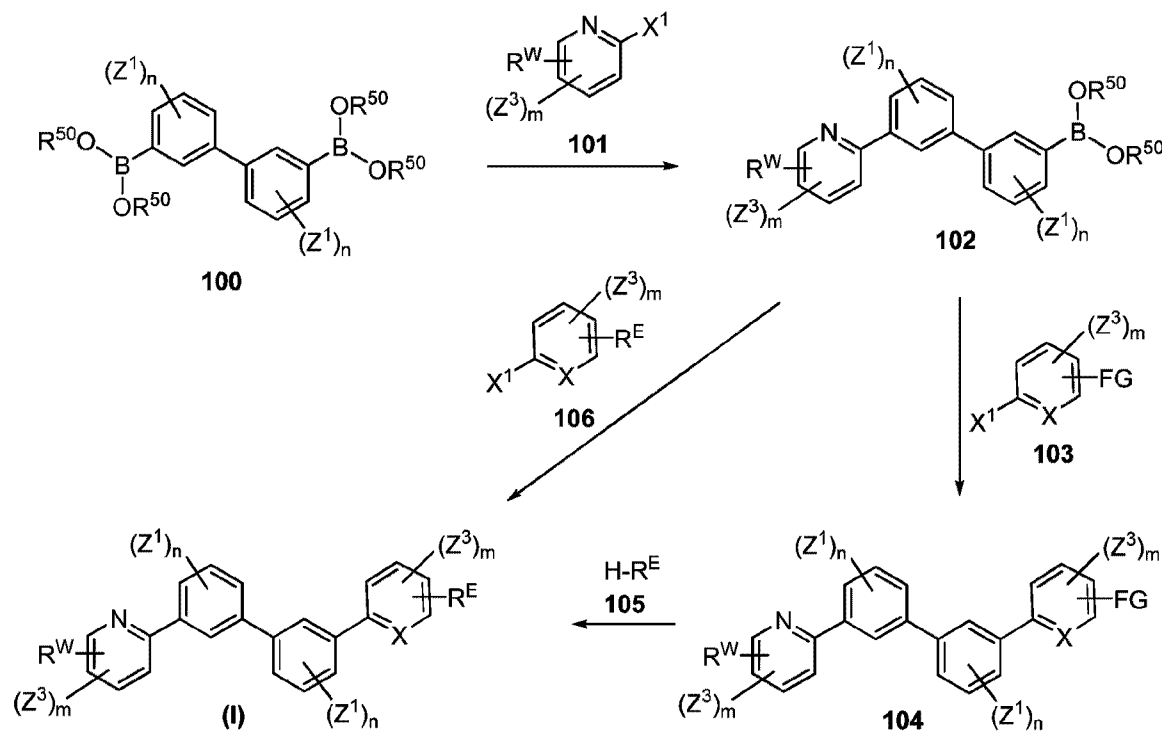
Scheme 1
