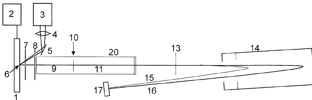
Figure 2 (prior art)
