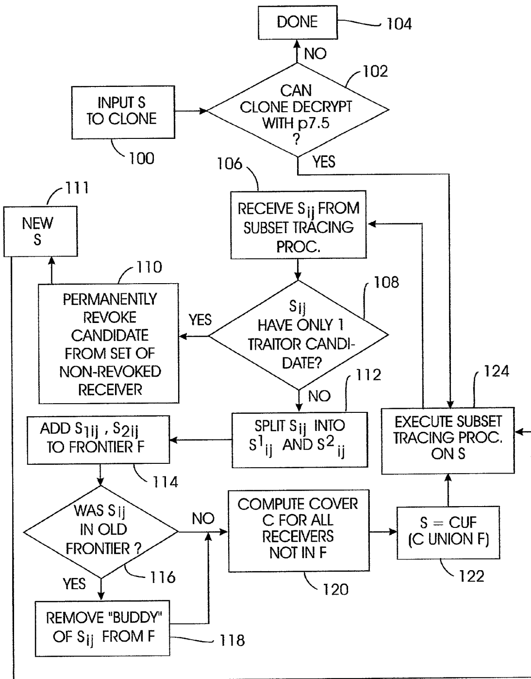
FIG. 15 TRACING ALGORITHM
