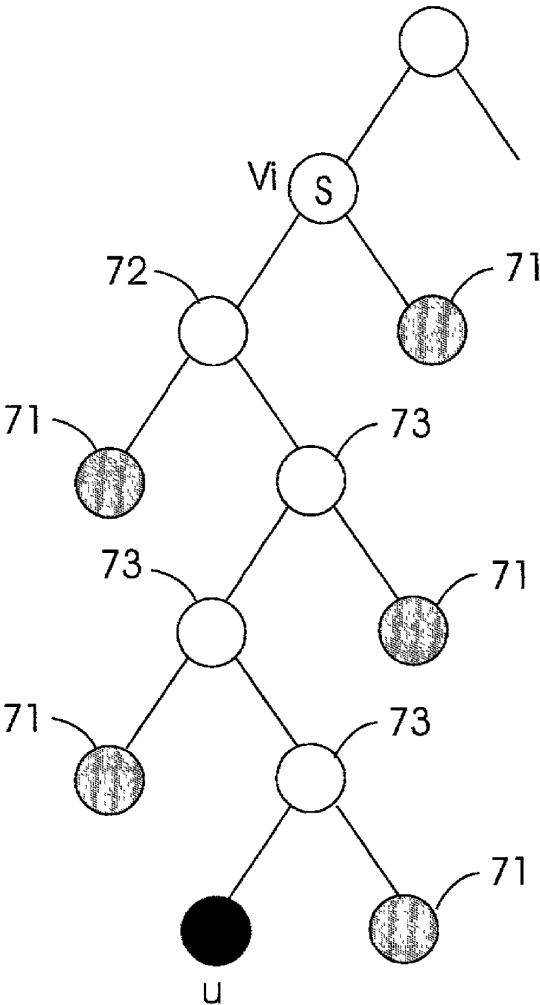
FIG. 14 - ASSIGNMENT OF LABELS SUBSET DIFFERENCE METHOD
