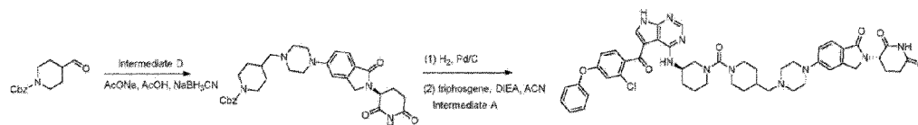
Scheme 7: Method for the preparation of reference compound 32
