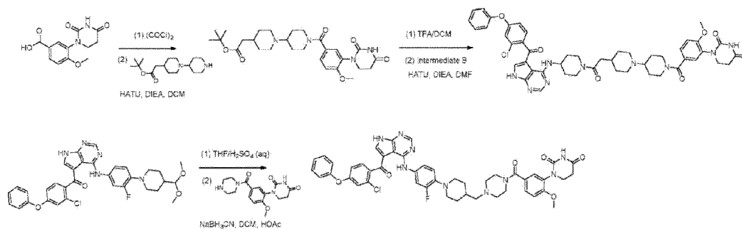
Scheme 14: Method for the preparation of reference compounds 73 and 74
