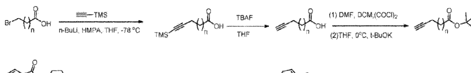
Scheme 8: Method for the preparation of reference compounds 35, 36, and 38
