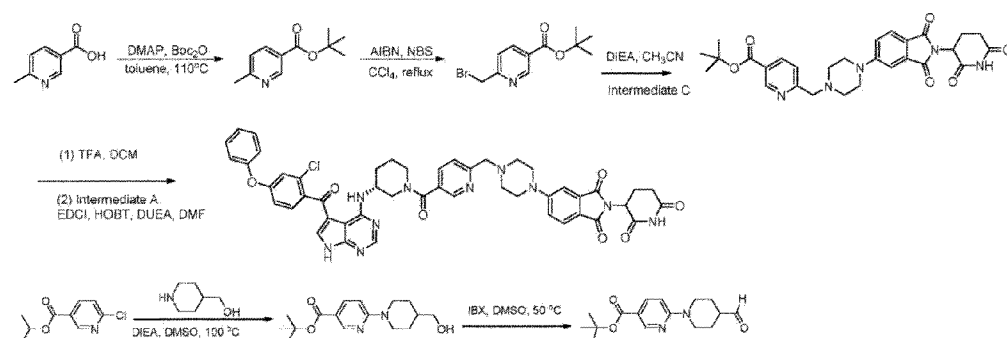
Scheme 5: Method for the preparation of reference compounds 9 and 10
