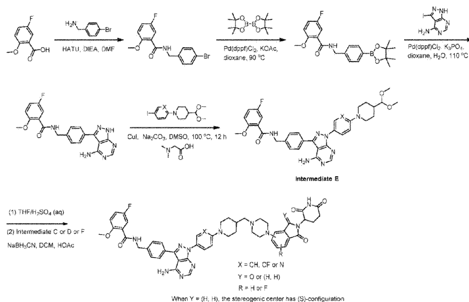
Scheme 11: Method for the preparation of compounds 49, 50, 51, 59, and 70
