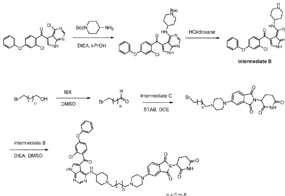
Scheme 6: Method for the preparation of reference compounds 12 and 18
