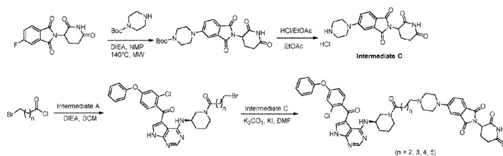
Scheme 3: Method for the preparation of reference compounds 7, 8, 11, and 19
