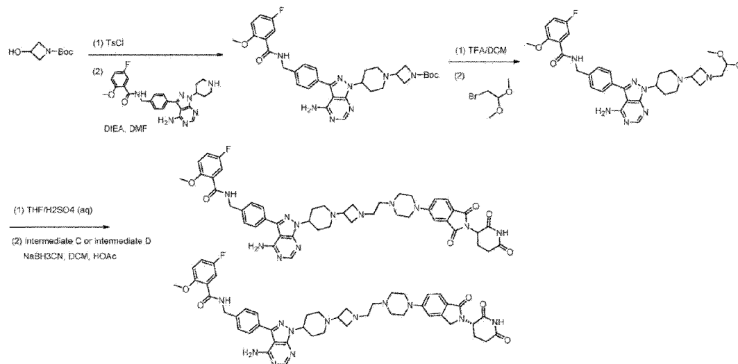
Scheme 16: Method for the preparation of compounds 86 and 87
