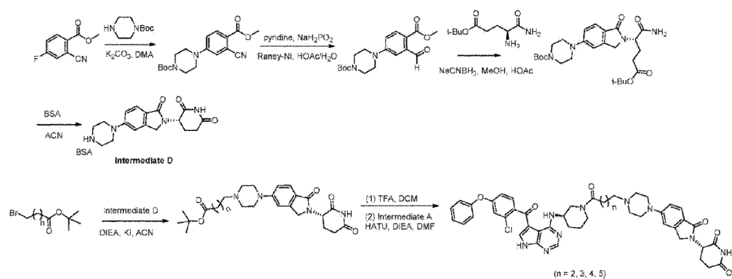
Scheme 5: Method for the preparation of reference compounds 9 and 10
