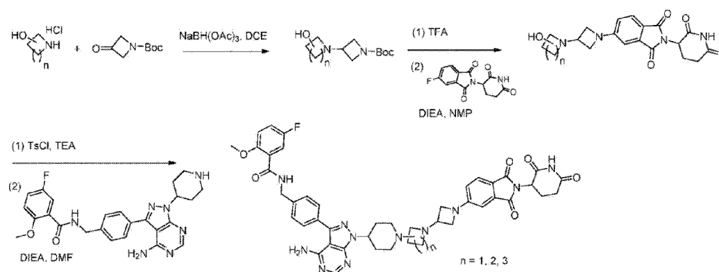
Scheme 15: Method for the preparation of compounds 83 and 84
