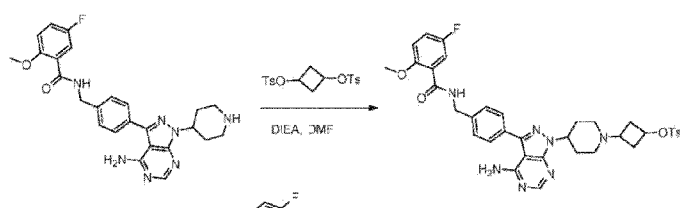
Scheme 17: Method for the preparation of compounds 88-91 and 100-101
