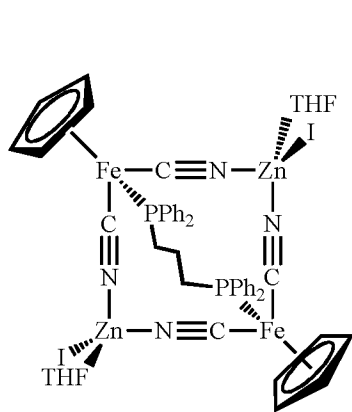
[\text{CpFe}(\mu\text{-CN})_2\text{ZnI}(\text{THF})]_2(\mu\text{-dppp}) DMC of iron and zinc
