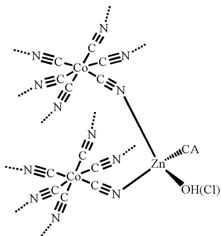
DMC of zinc and cobalt \text{Zn}_3\text{Co}(\text{CN})_6 \cdot x\text{ZnCl}_2 \cdot y\text{H}_2\text{O} \cdot z\text{CA} CA: Complexing agents
