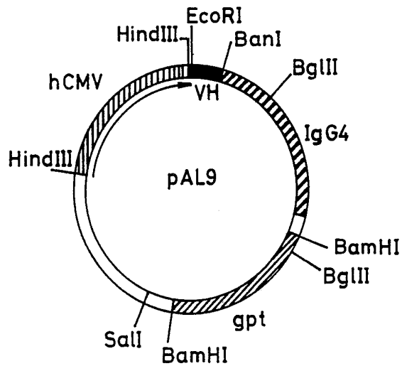
pAL9, CHIMAERIC HEAVY CHAIN EXPRESSION VECTOR IgG4 isotype
