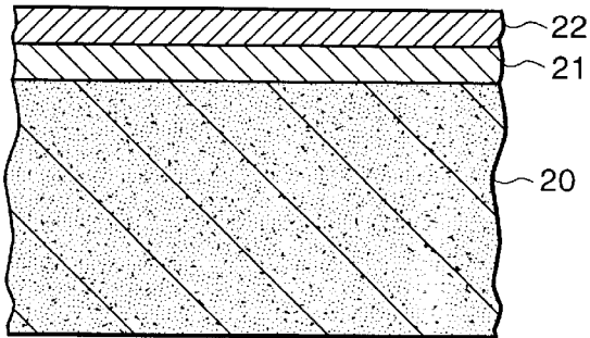
Fig. 1 (PRIOR ART)
