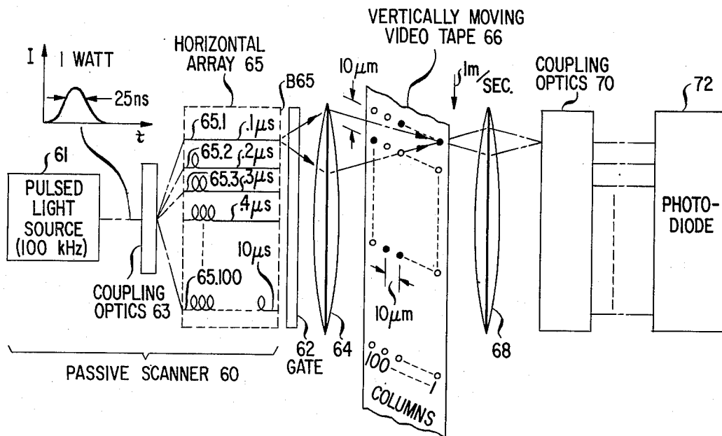
FIG. 3 MEMORY SYSTEMS
