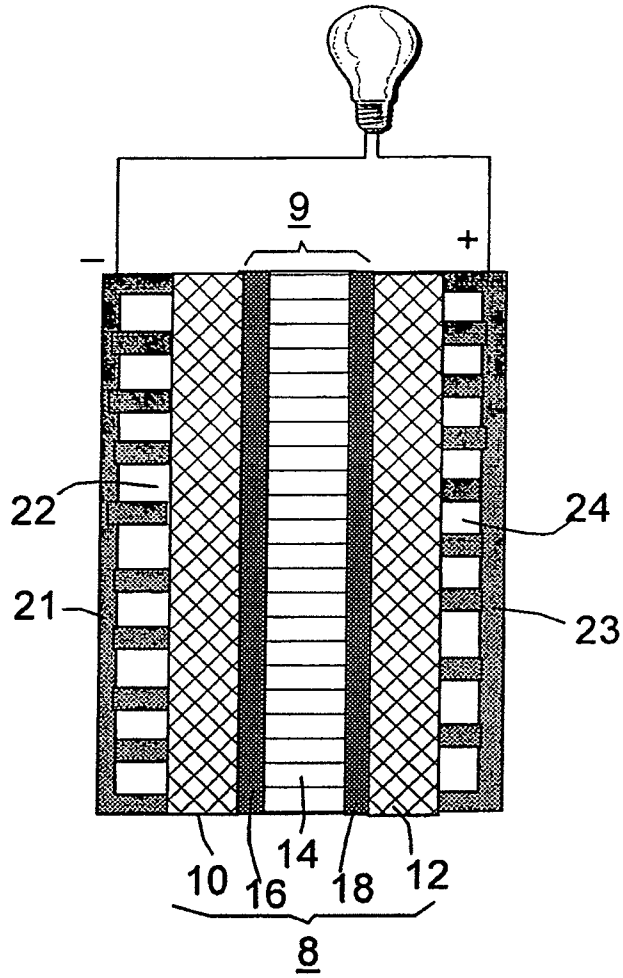
FIG.1 (Prior Art)
