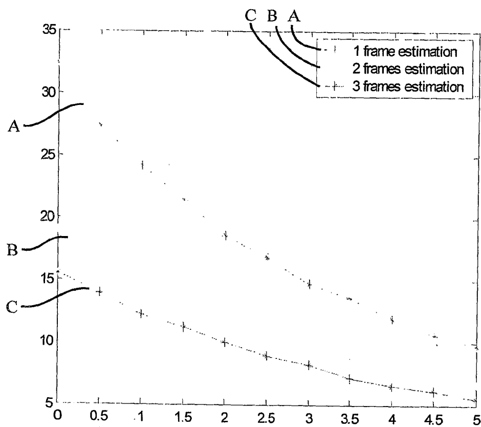
STD of the Doppler estimation error vs. SNR for several numbers of used UL
