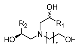
Formula (13b-6)
