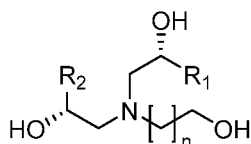
Formula (13b-2)
