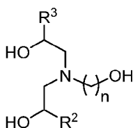
Formula (14-2)
