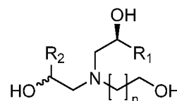
Formula (13b-9)
