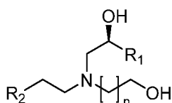
Formula (13a-2)
