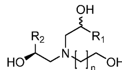
Formula (13b-6)
