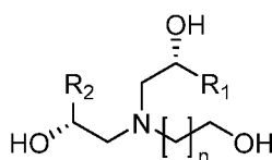
Formula (13b-2)
