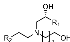
Formula (13a-3)
