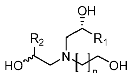
Formula (13b-8)
