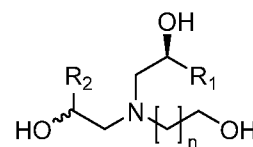
Formula (13b-9).
