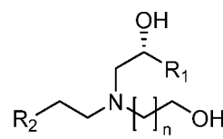
Formula (13a-3)
