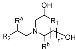
Formula (13*)
