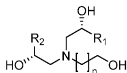
Formula (13b-2)
