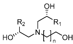
Formula (13b-2)
