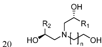
Formula (13b-4)
