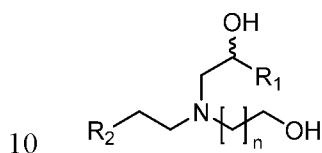
Formula (13a-1)
