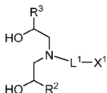
Formula (14)
