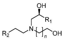
Formula (13a-2)
