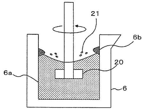
(KR DESULFURIZATION PROCESS)
