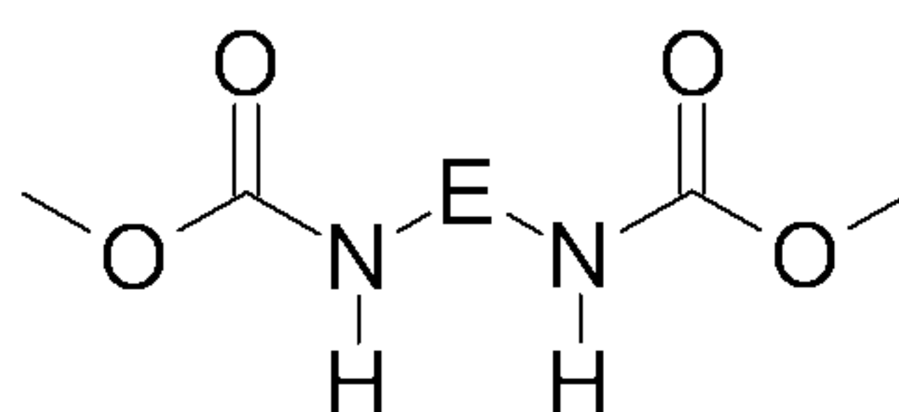
formula (U-1)
