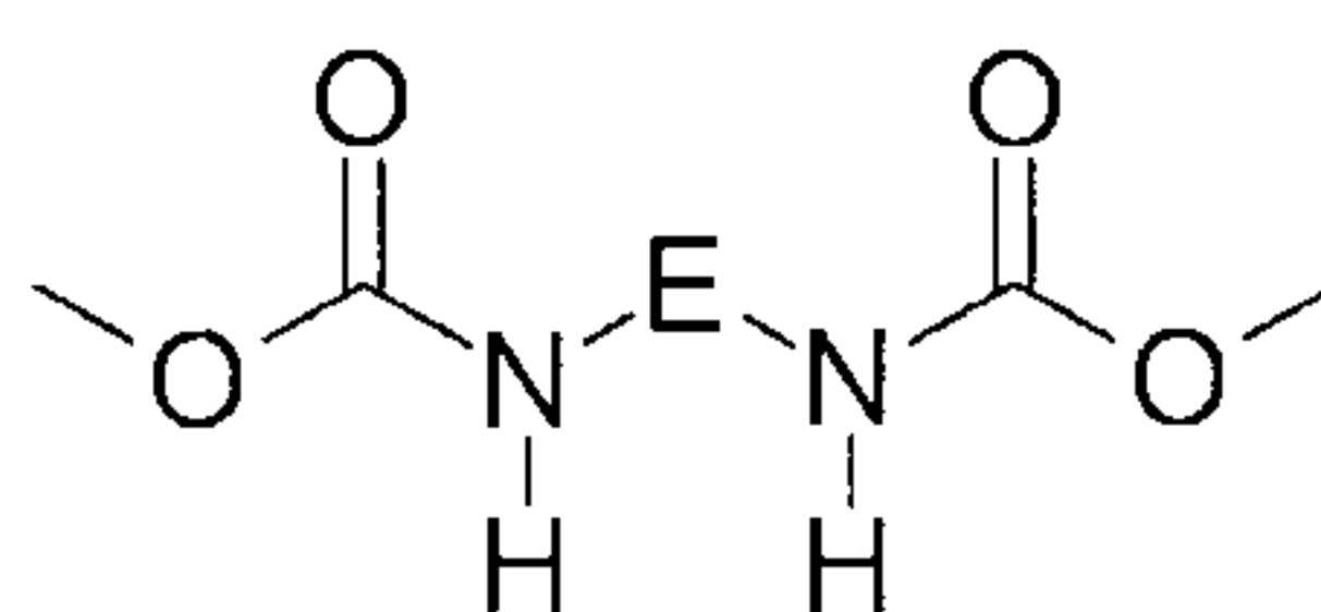
formula (U-1)
