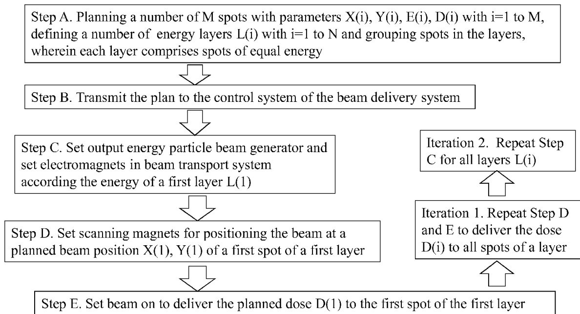
Fig. 3 (Prior Art)
