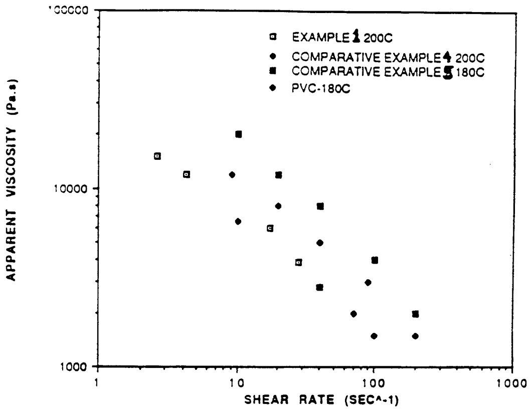
FIGURE 1: VISCOSITY VERSUS SHEAR RATE FOR RESIN COMPOSITIONS
